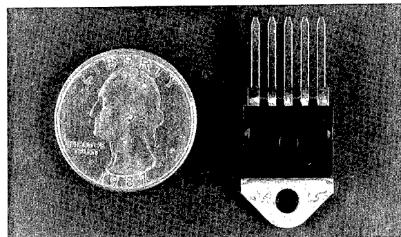
Miniaturization has allowed SDI to make great technological advances. Pictured is a Metal Oxide Semiconductor (MOS) -Controlled Thyristor (MCT) switching device.
