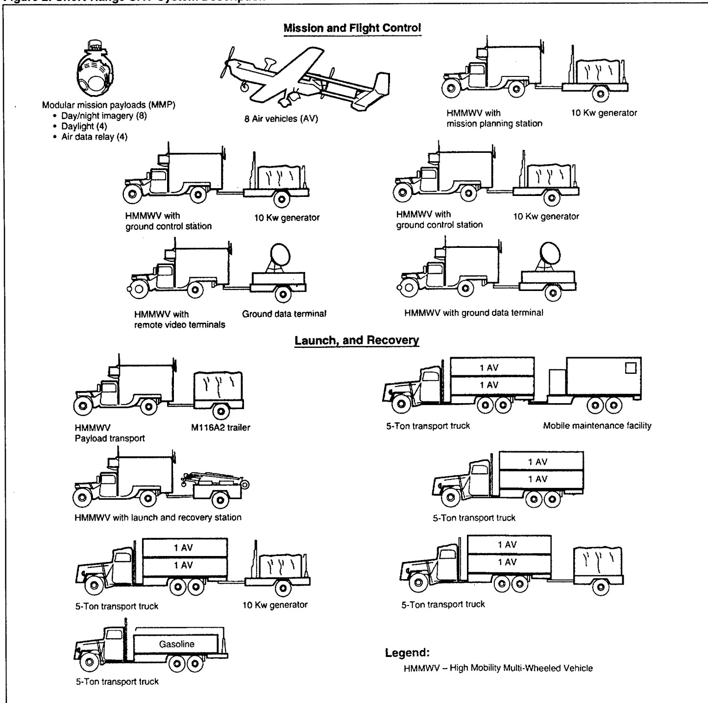
Figure 2: Short-Range UAV System Description
