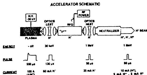
Fig. 2. A conceptual view of the accelerator.
