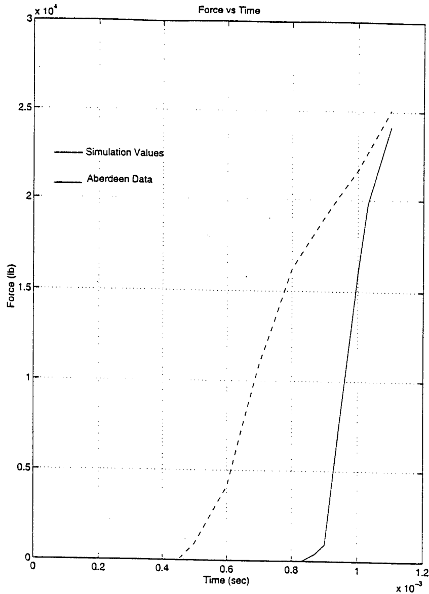
Figure 8.1 Comparison of Aberdeen test data and FEM data.
