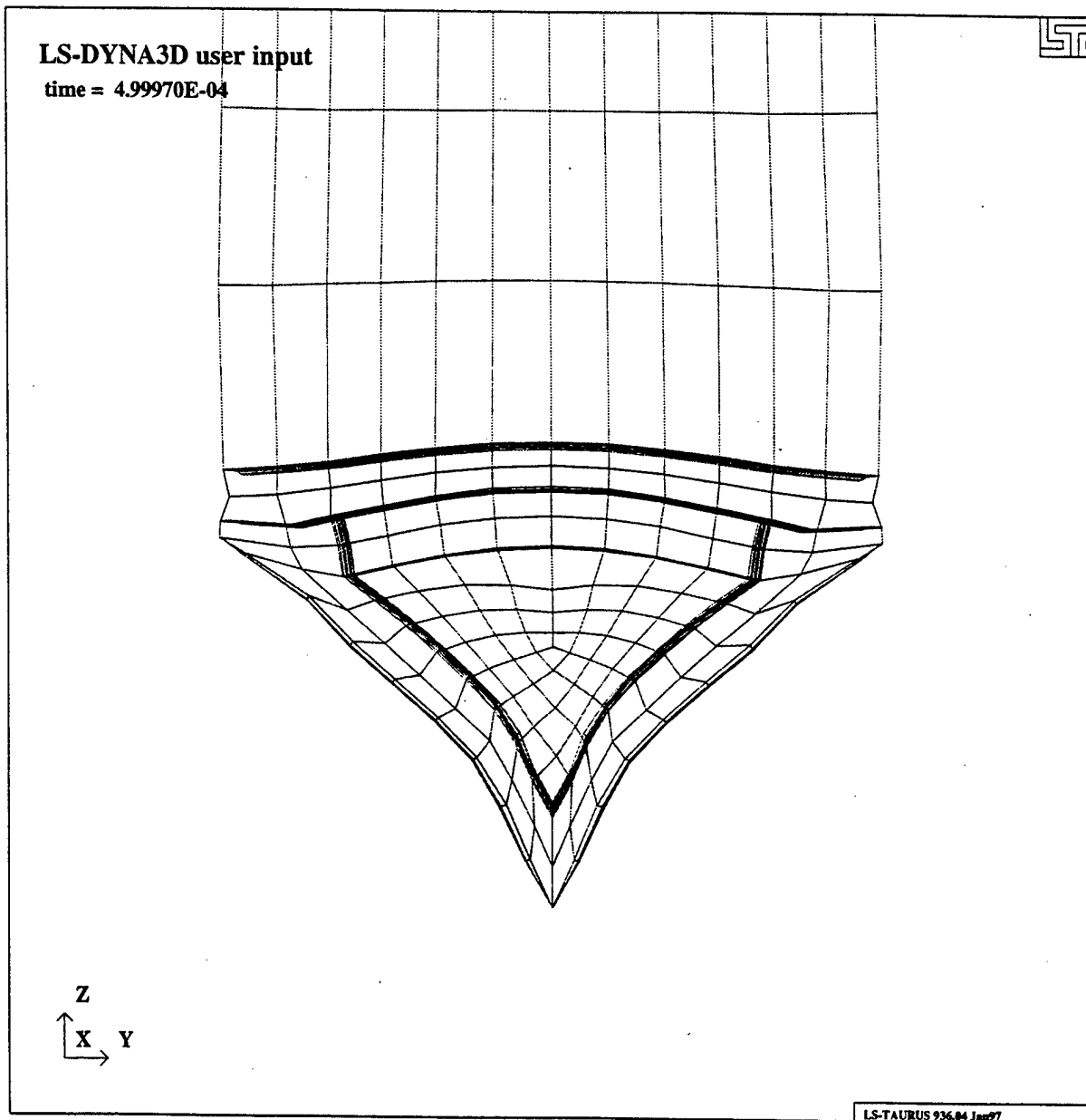
Figure 8.3 Deformation of the boot at approximately 0.5 milliseconds.
