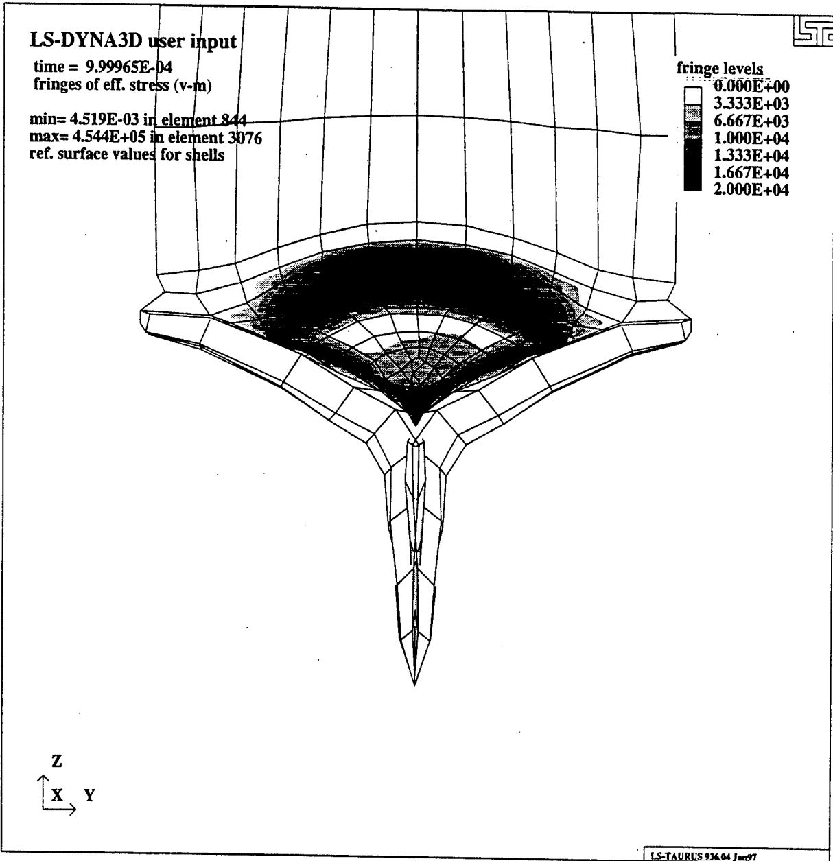
Figure 8.8 Von Mises stress across the boot at approximately 1.0 milliseconds.
