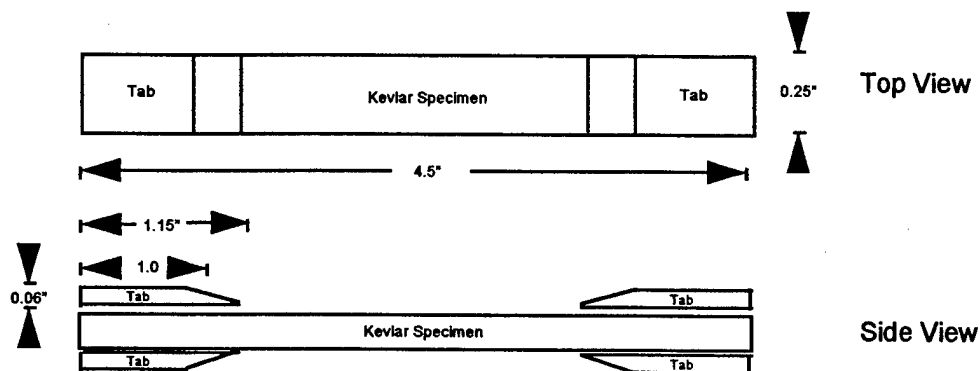
Figure 5.5 Diagram of tab dimensions.
