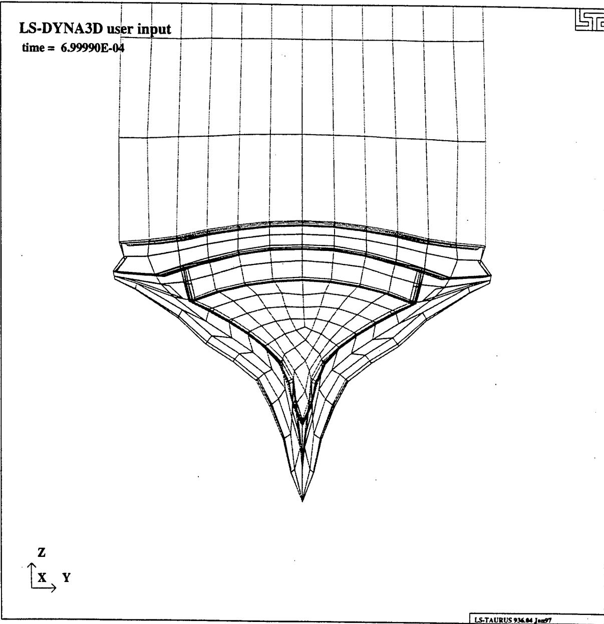
Figure 8.4 Deformation of the boot at approximately 0.7 milliseconds.
