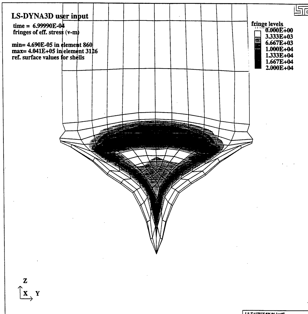
Figure 8.7 Von Mises stress across the boot at approximately 0.7 milliseconds.
