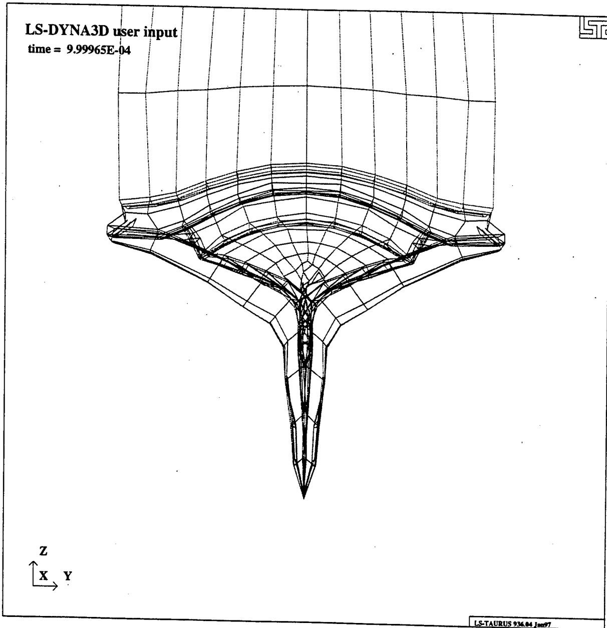
Figure 8.5 Deformation of the boot at approximately 1.0 milliseconds.
