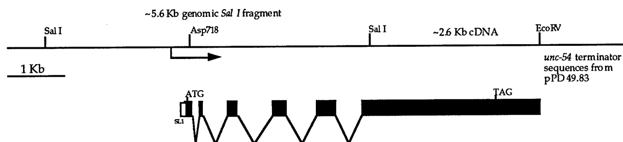
Figure 5. Schematic of rok-1 minigene. Above is the genomic clone, below a full length cDNA.
