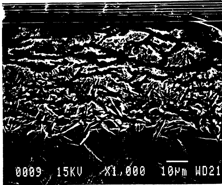
Figure 33 - Microstructure of hydride layer on the grade 2 titanium sample surface after the sample was charged in 3.5%NaCl solution (pH=1) at -1400 mV SCE and 70°C for 168 hours.
