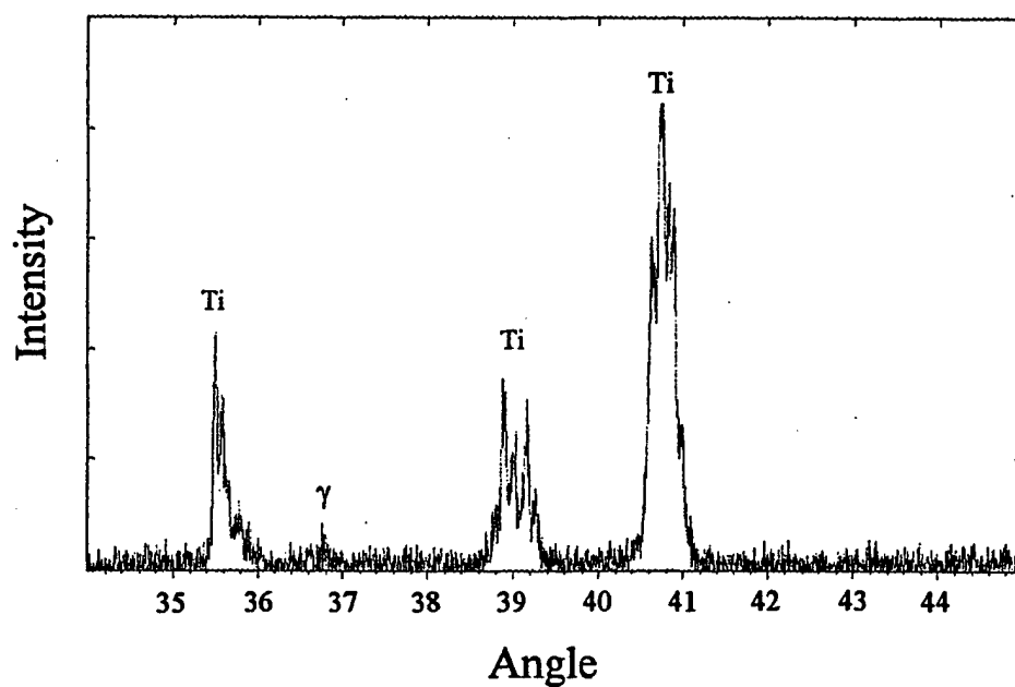
Figure 38 - XRD pattern obtained from LP samples with pickled surface after being charged at a potential of -1800 \text{ mV}_{SCE} .
