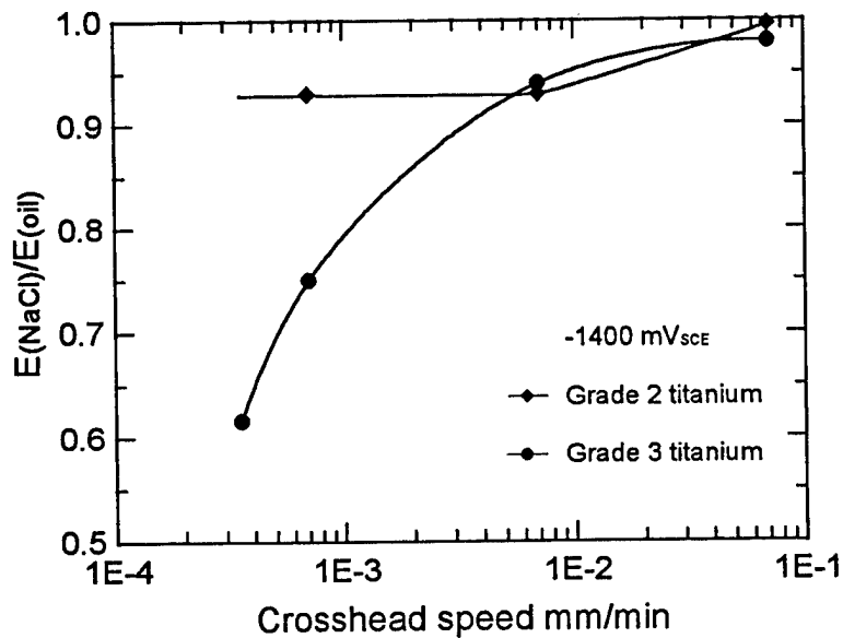
Figure 42 - The ratio of the elongation to failure in 6%NaCl (pH=1) to that obtained in oil plotted as a function of applied crosshead speed for grade 2 and grade 3 titanium at 70°C.
