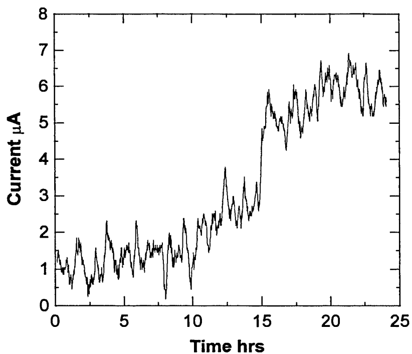
Figure 37 - Hydrogen permeation current plotted as a function of time for the LP sample with pickled surface at -1800 \text{ mV}_{SCE} .
