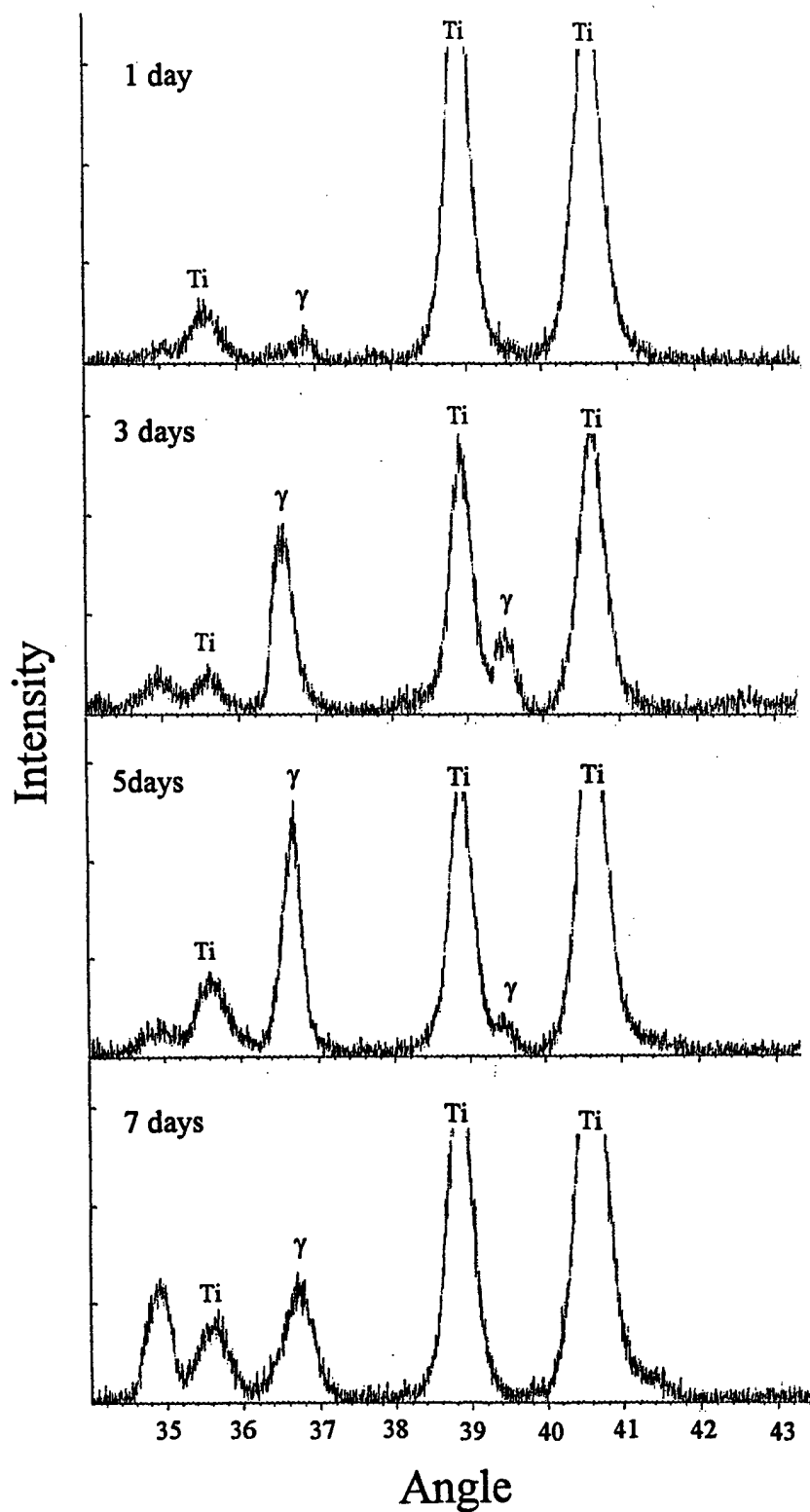
Figure 32 - XRD pattern obtained from grade 2 titanium samples after being charged at a potential of -1400 mV SCE in 3.5%NaCl solution (pH=7) at 70°C for up to 168 hours.
