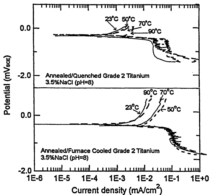
Figure 18 - Polarization curve for heat-treated grade 2 titanium at various temperatures in 3.5%NaCl solution with pH=8.
