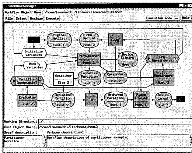
Fig. 7. Partitioner workflow.
