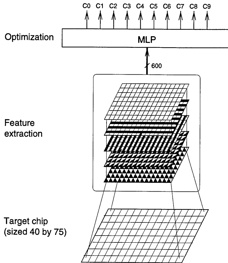
Figure 5. A fully connected network classifier for ATR.
