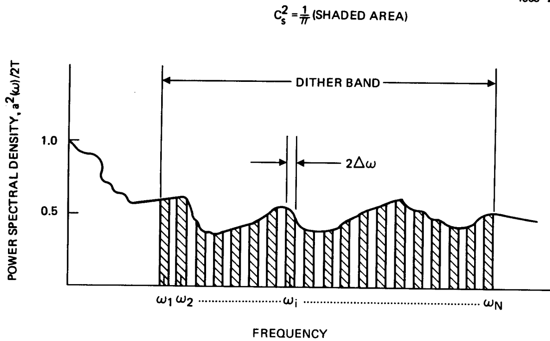
Figure 23. Power spectrum of an arbitrary modulation function.
