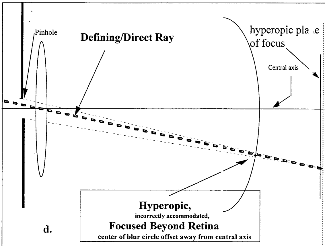
Figure 12d. Expanded illustration to clarify the locus of the off-axis end point of retinal stimulation for hyperopic accommodation.
