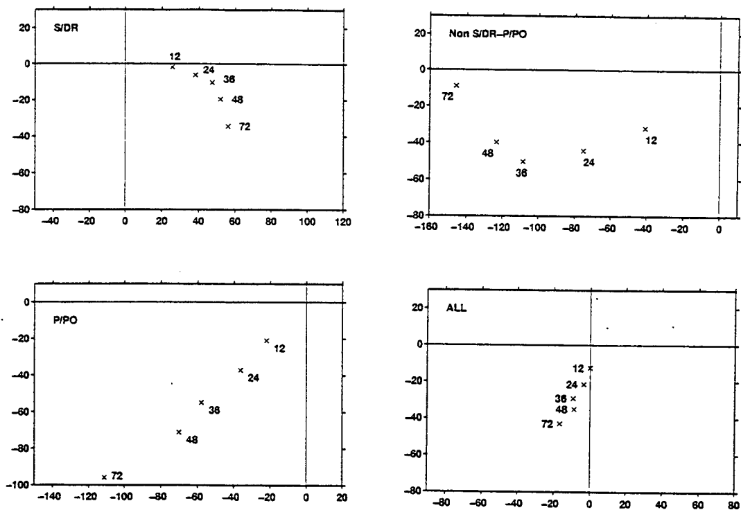
Figure 15. Mean positions of the unadjusted NOGAPS track forecast errors (n mi) from 12 h through 72 h relative to the actual TC position (0,0) for S/DR, P/PO, other than S/DR or P/PO, and all TCs.
