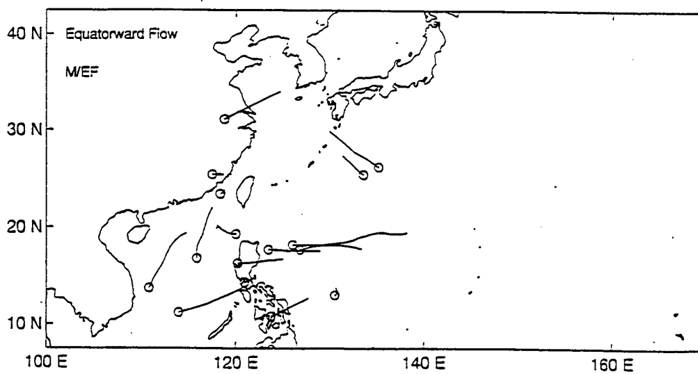
Figure 10. Storm tracks as in Figure 4, except in Multiple (M) synoptic pattern and the Poleward Flow (PF), and Equatorward Flow (EF) regions (From CEB98).
