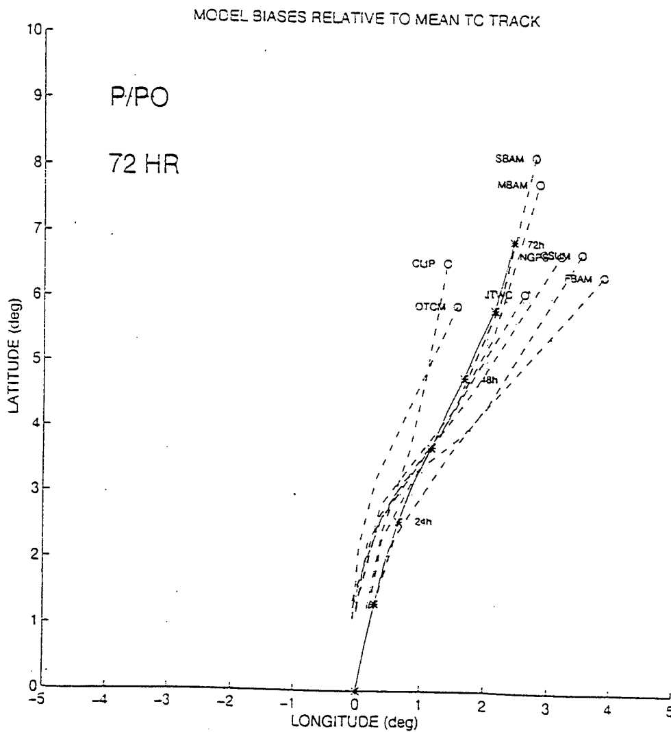
Figure 1b. Track forecast biases of several modeling techniques relative to mean (actual) P/PO tracks (provided by L. Carr).
