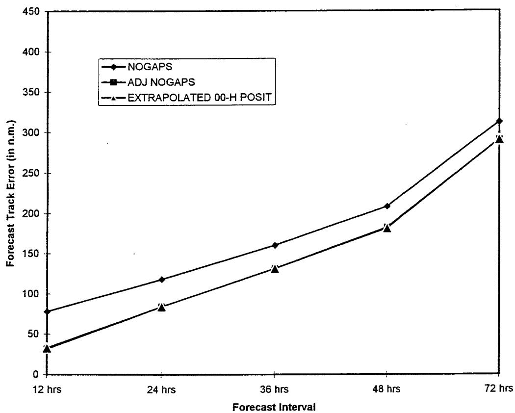
Figure 16. NOGAPS track forecast errors as in Fig. 14 with the full 3/3 development sample of PR/ALL synoptic pattern/regions, except using an extrapolated NOGAPS starting position, rather than the CARQ position. The 2/3 development sample is not shown.
