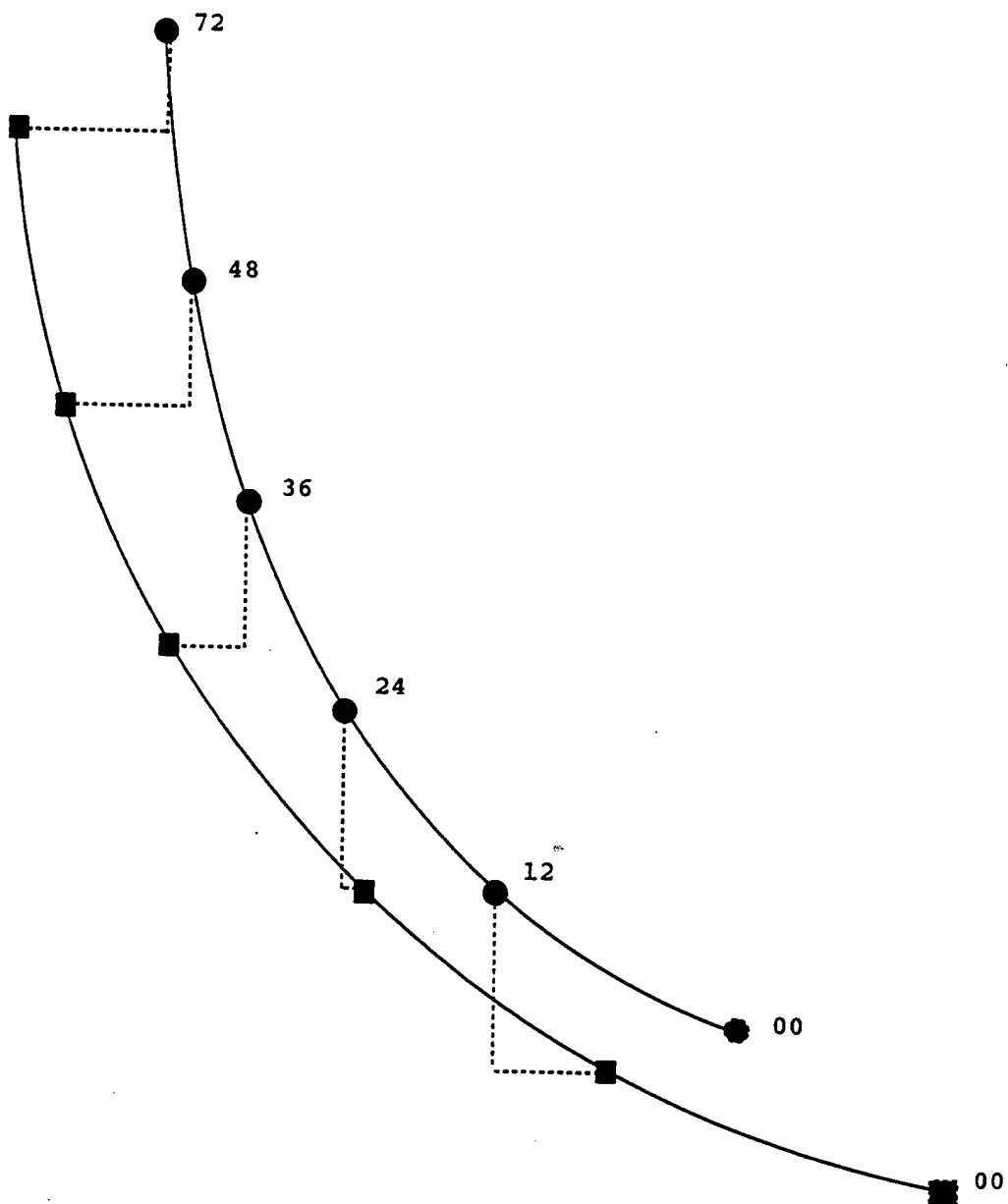
Figure 11. Schematic of the 10 predictands, which are the zonal and meridional displacements necessary to adjust the NOGAPS forecast track (circles) to the best track (squares).
