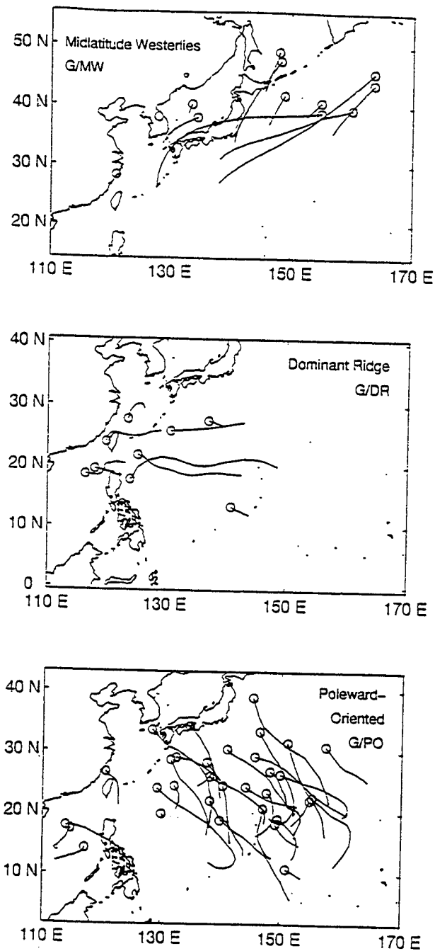
Figure 8. Storm tracks as in Figure 4, except in the monsoon Gyre (G) synoptic pattern and the Midlatitude Westerlies, Dominant Ridge, and Poleward-Oriented regions (From CEB98).
