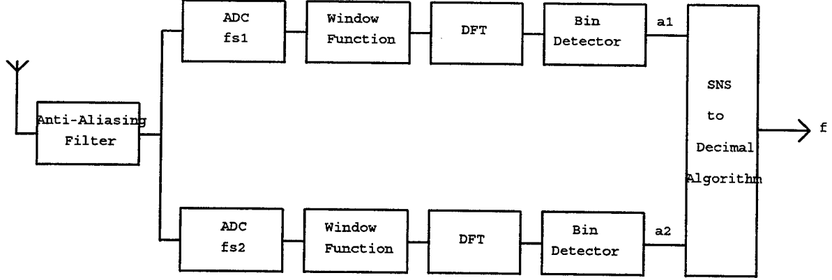
Figure 2: Block Diagram of a Two Channel Receiver Architecture.
