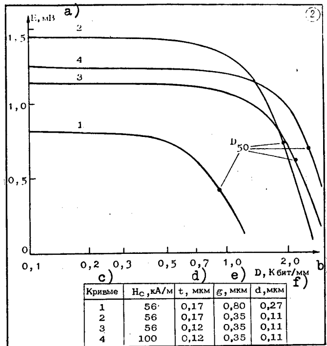
Figure 2. Relationship of amplitude, E , to recording density, D , at different values of H_c , t , g and d (reference 9).
