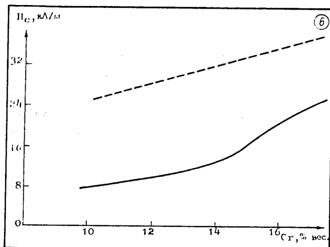
Figure 6. Relationship of strength of coercivity, H_c , of cobalt-chromium films on glass substrates (continuous line) and on a chromium sublayer (dotted line) to chromium content in films.
