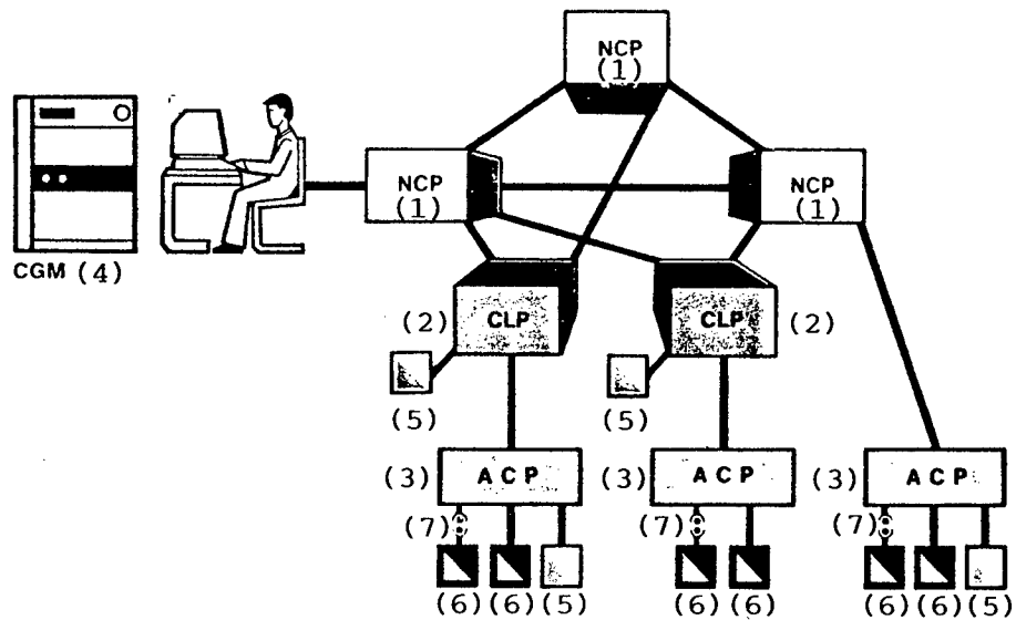
Fig 3 - ITAPAC network.
