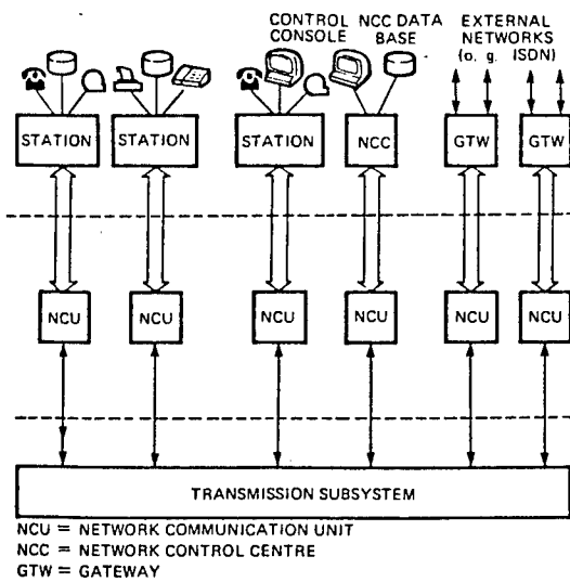
Fig. 1 - LION reference architecture.
