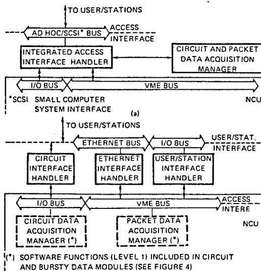
Fig. 5 - Access interface modules towards NCU: (a) integrated circuit/packet access interface; (b) specialized (service oriented) access and user interfaces.
