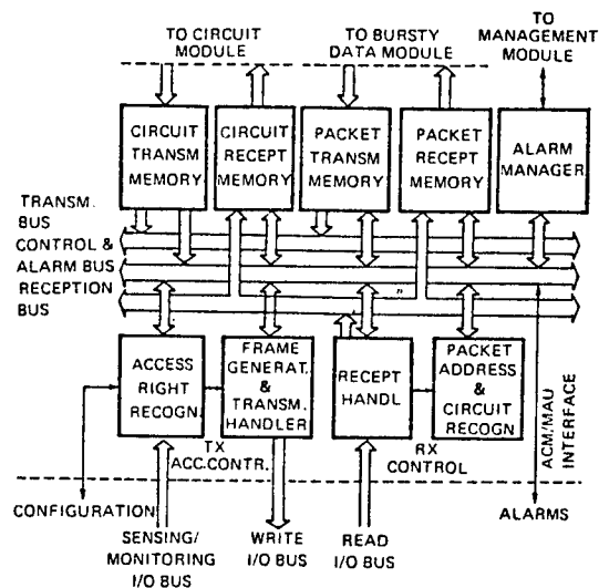
Fig. 6 - Access control module and I/O memories block diagram.
