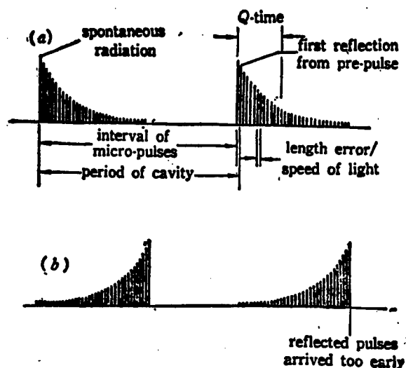
Figure 2. Wave Shape of Optical Pulses From Spontaneous Radiation
