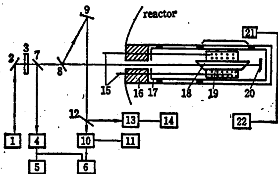
Figure 1. Experimental Arrangement
