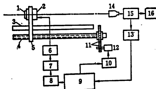
Figure 4. Principle Schematic of the Cavity Adjustment Device
