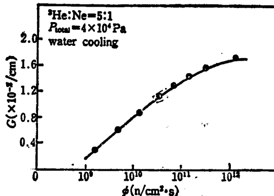
Figure 3. Gain Coefficient as a Function of Neutron Flux
