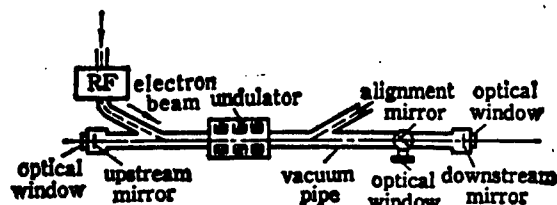
Figure 1. Principle Schematic of FEL Cavity Structure
