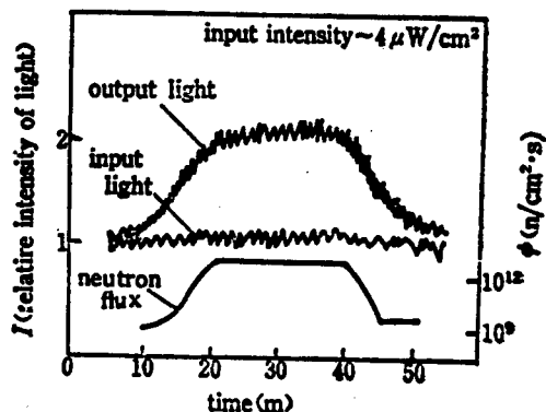
Figure 2. Time Dependence of Input Intensity, Output Intensity and Neutron Flux
