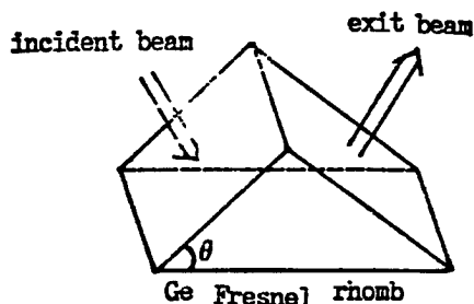
Fig. 4 The phase shift with each internal reflection
