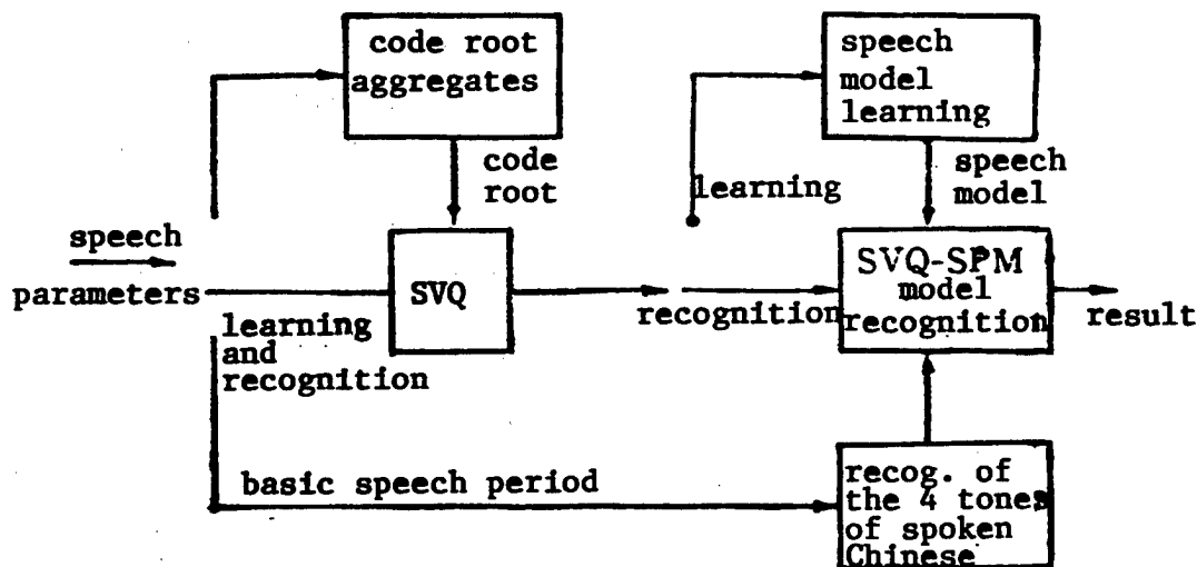
Figure 1. Schematic of Syllable-Recognition Subsystem
