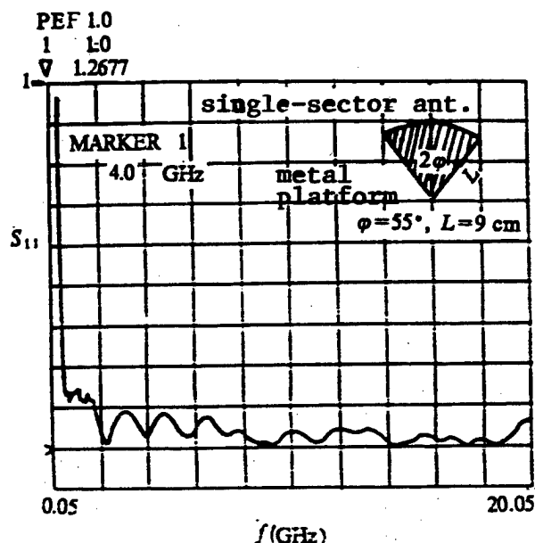
Figure 3. Measured Input SWR of V-Shaped Conical Receiving Antenna
