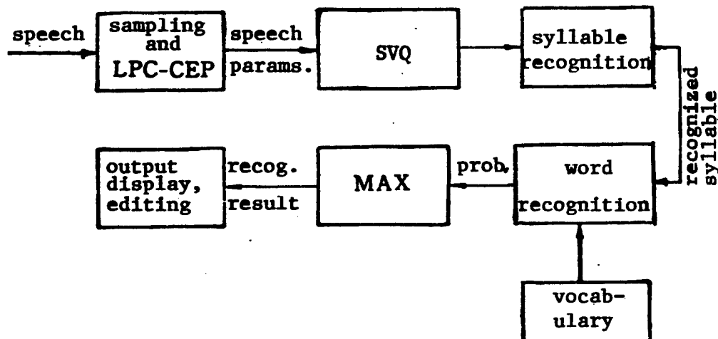
Figure 2. Schematic of Overall Speech Recognition System
