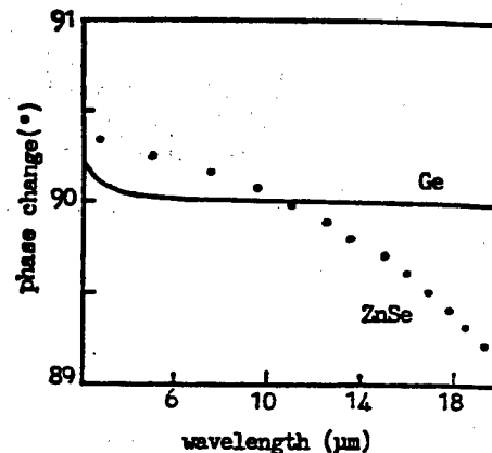
Figure 3. The Chromatic Curve of 1/4λ Fresnel Rhomb
