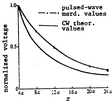
Figure 5. Exper. Results for Pulsed-Wave Transmission Characteristics
