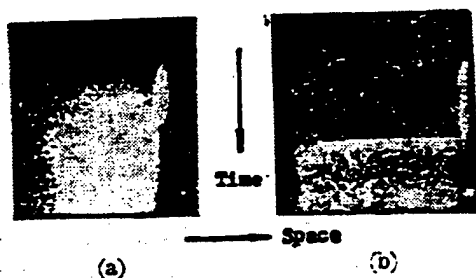
Figure 6. Luminescence Signal at the Back Surface of Aluminum Foil Obtained by the Streak Camera. (a) Only principal focusing lens; (b) Principal focusing lens with a regular hexagonal lens array
