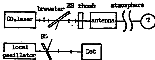
Figure 1. Basic Diagram of CO 2 Laser Heterodyne Receiving
