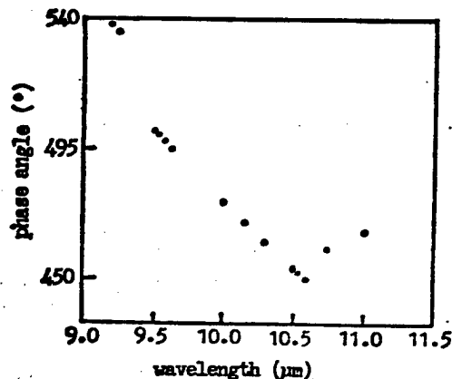
Figure 2. The Distribution of 5/4λ CdS Wave Plate Near 10.591 μm
