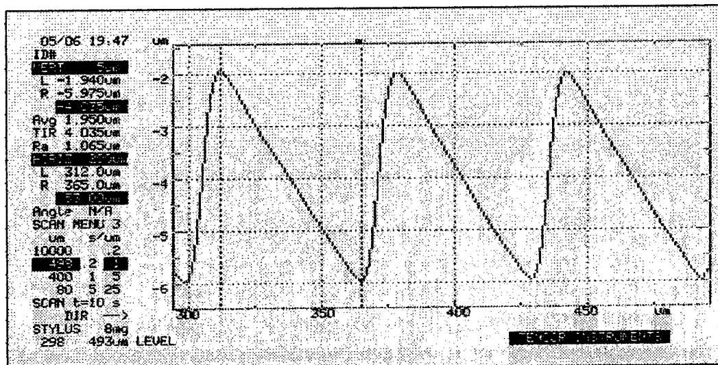
Figure 13. Profilometry scan of the off-axis field grating lens fabricated in InAs, shown in Figure 12. Notice the smooth, continuous surface of each of the diffraction zones, and the linearity of the blazed surface. The etch depth of this sample was 4.035 \mu\text{m} . It was etched using an ion mill with gas flow mixtures Ar:54 % and O 2 :46 %, yielding a 1.2:1 selectivity.
