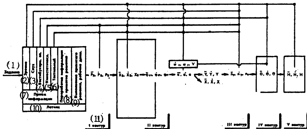
Key: 1. Assignment 2. Vision 3. Hearing 4. Vestibular apparatus 5. Kinesthetic 6. Tactile 7. Information reception 8. Information processing and decision making 9. Fulfillment of adopted decision, working movements 10. Pilot 11. Loop
