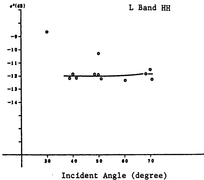
Fig. 4 Dependency of on incidence in case of field in Tsukuba
