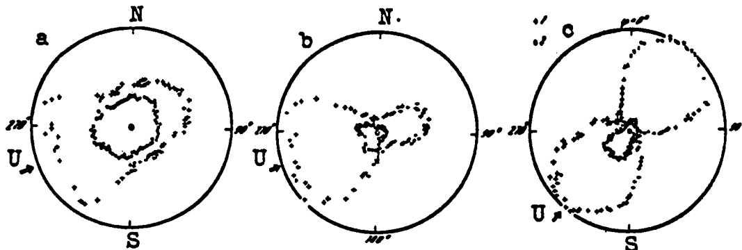
Fig. 4. Azimuthal characteristics \alpha(\varphi) at \theta = 57^\circ : crosses - V-polarization, dots - H-polarization; (a) calm, U = 0 , (b) steady wind, U = 8 \text{ ms}^{-1} , (c) gusty wind, U = 8 - 8 \text{ ms}^{-1}
