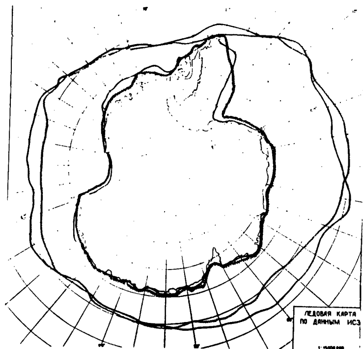
Fig. 4 Extremal boundaries of drift-ice in season ~~~~~ 1982-83 and — 1983-84
