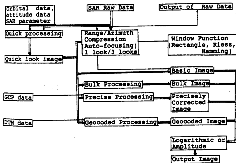
Fig. 2 Data Processing Flow of JERS-1 SAR data
