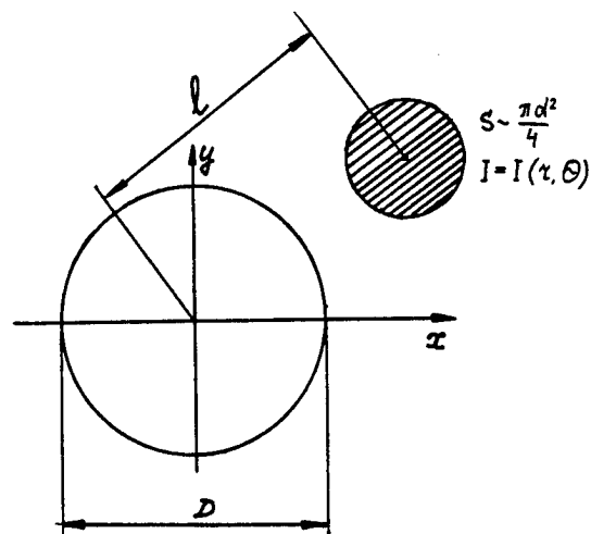
Fig. 1. Horizontal cross-section of the probing geometry.
