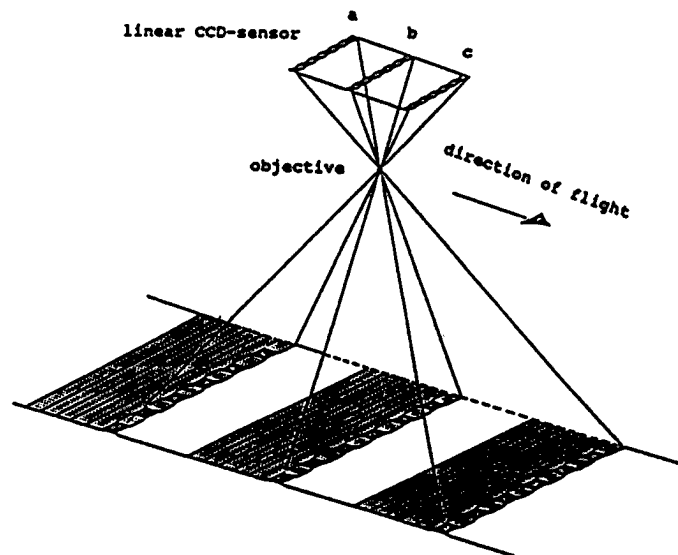
Fig. 1 Image Recording Using a Three Line Scanner
