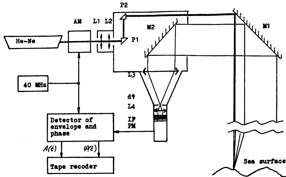
Fig. 3. Experimental set-up.
