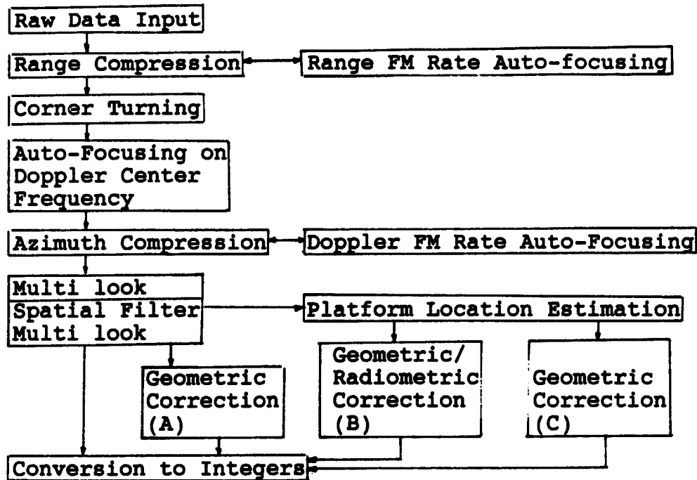
Fig 1. Data Processing Flow of SAR-580 Data
