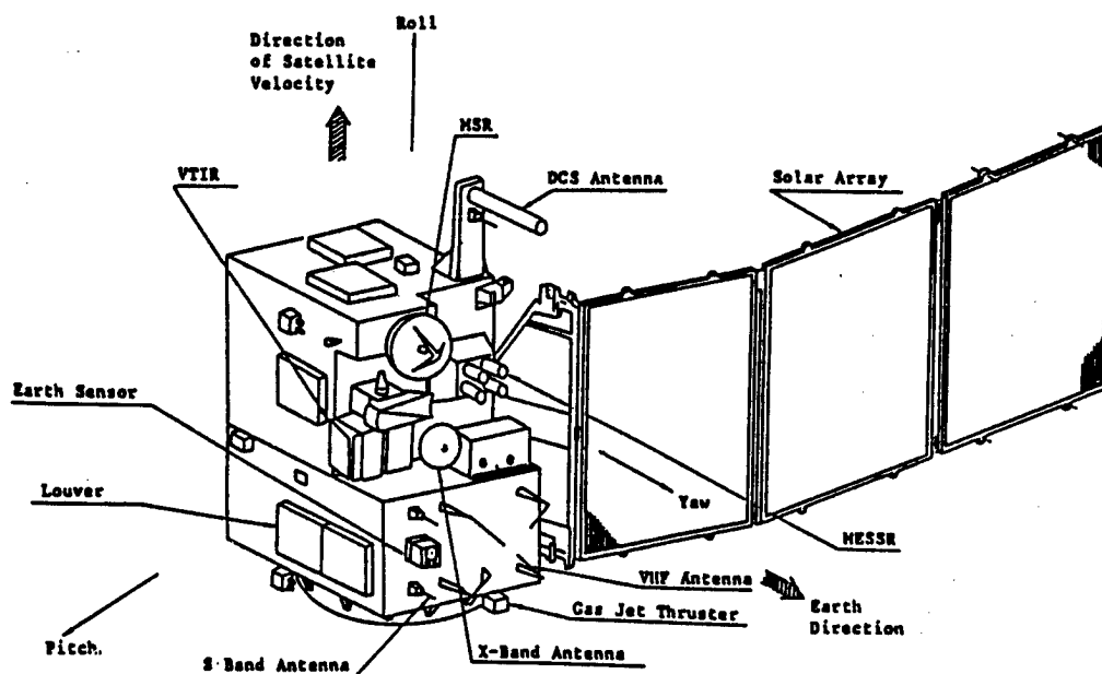
Fig. 1 Profile of MOS-1
