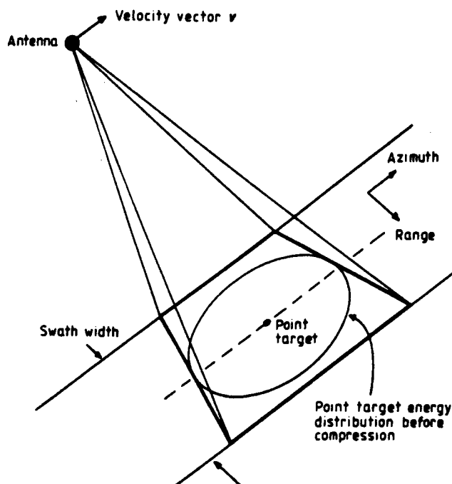
Fig. 1. Basic SAR Geometry
