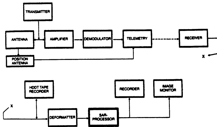
Fig. 2. Block Diagram of SAR System
