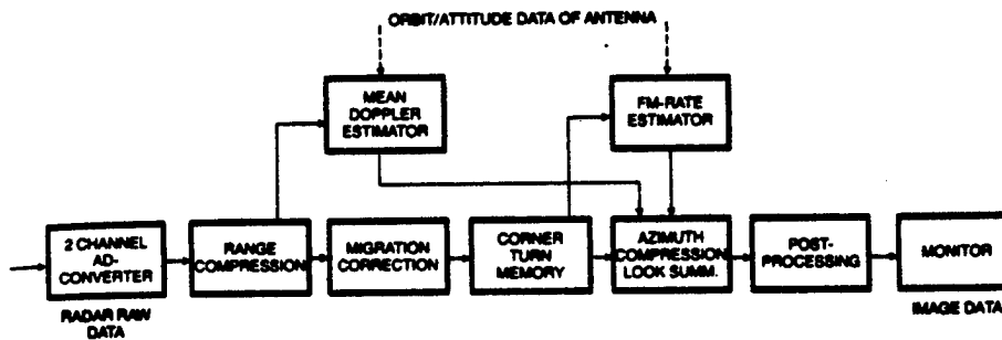
Fig. 3. SAR Processor Functions
