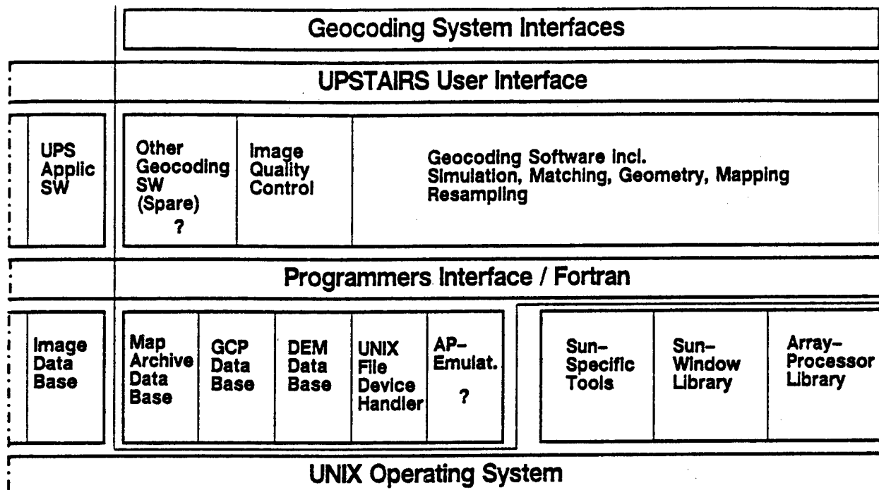
Fig. 3 Geocoding Image Processing System Software Layers
