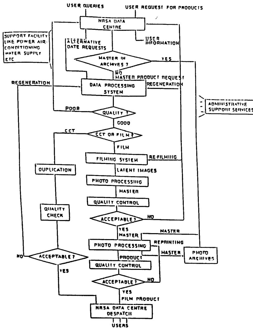
Fig. 3 Data Products Generation Flow
