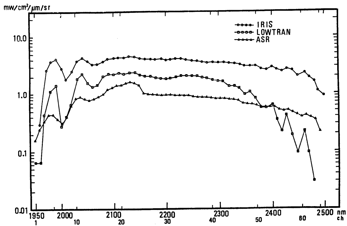
Fig. 4 Radiance by ASR, IRIS, and LOWTRAN 5
