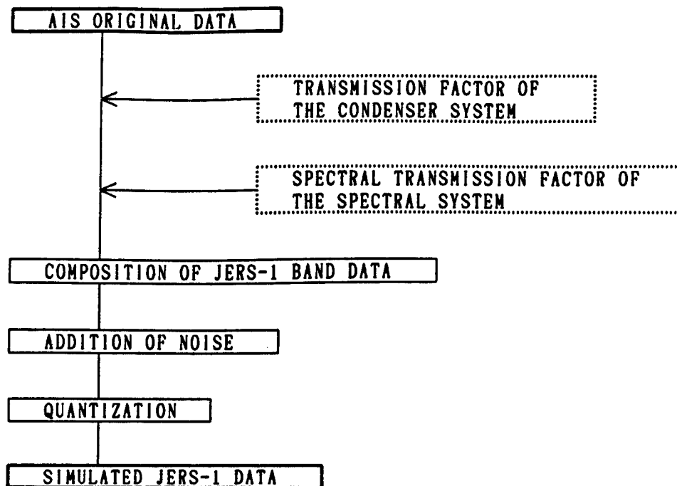
Fig. 2 Flow Chart of JERS-1 Data Simulation
