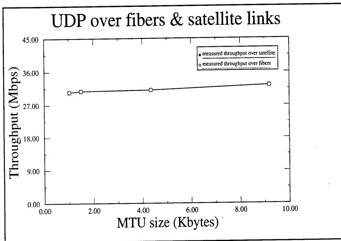
Figure 11: Application throughput with UDP over fibers and satellite links
