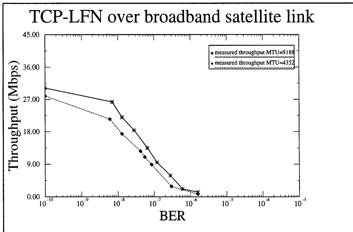
Figure 10: Application throughput with TCP-LFN over degraded satellite link
