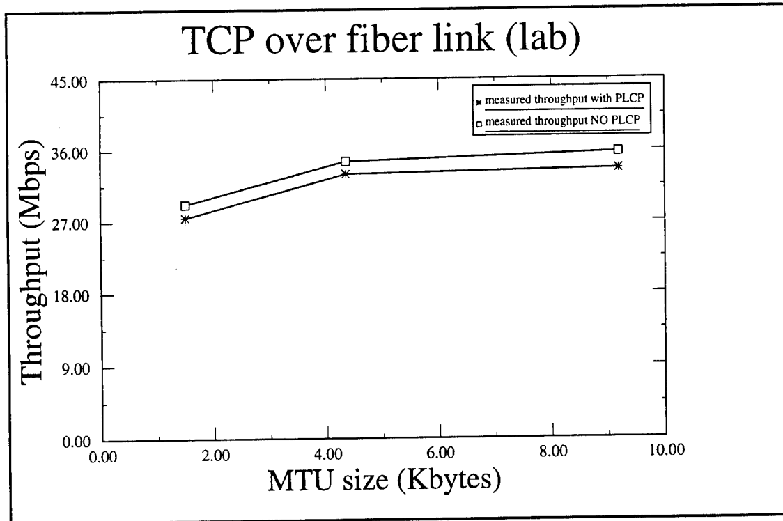
Figure 7: Application throughput with TCP over fibers
