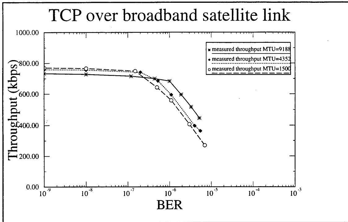
Figure 9: Application throughput with TCP over degraded satellite link
