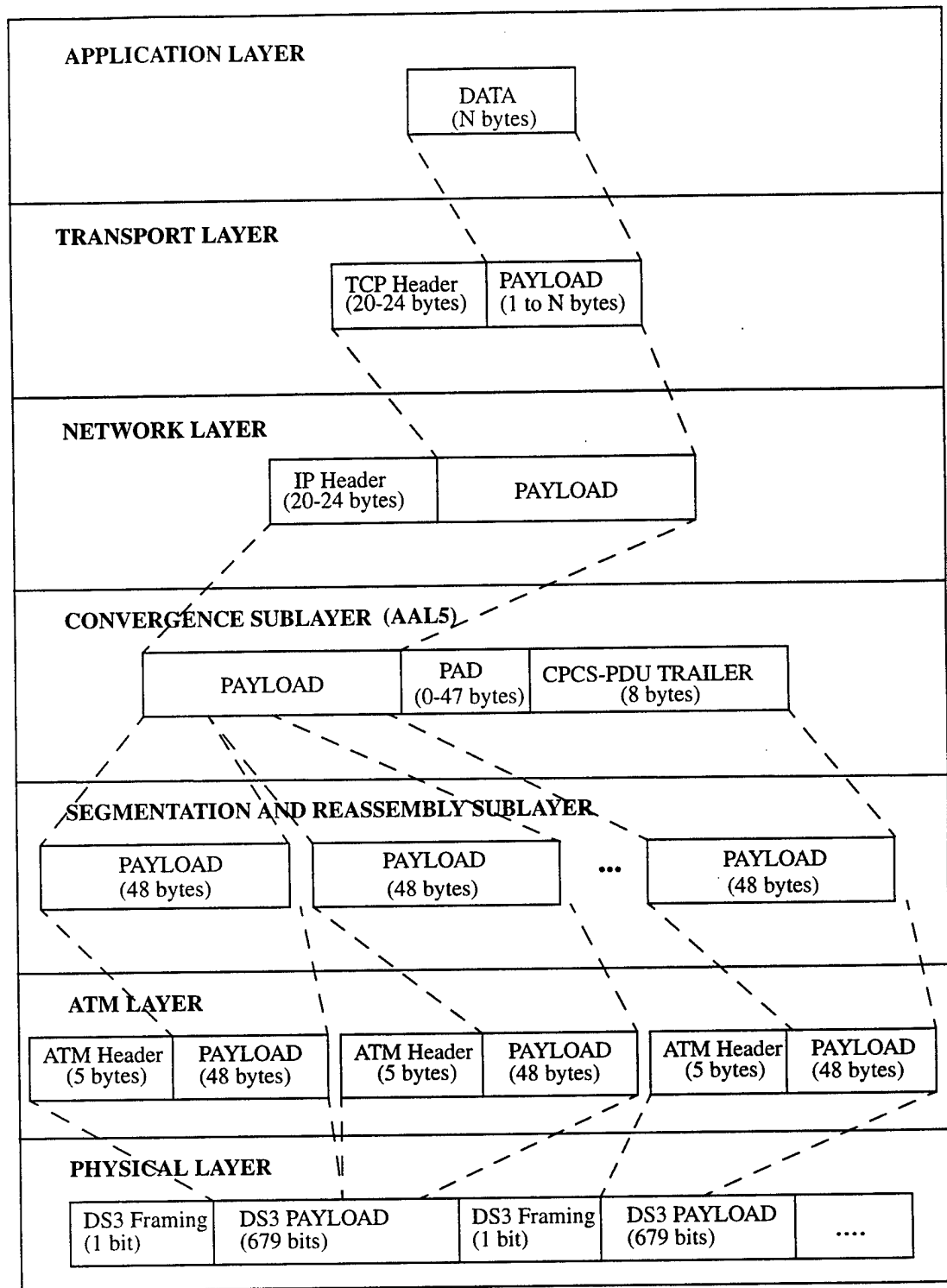
Figure 4: Protocol Overhead
