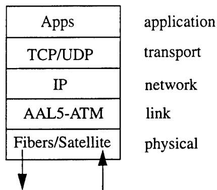
Figure 3: Protocol Stack
