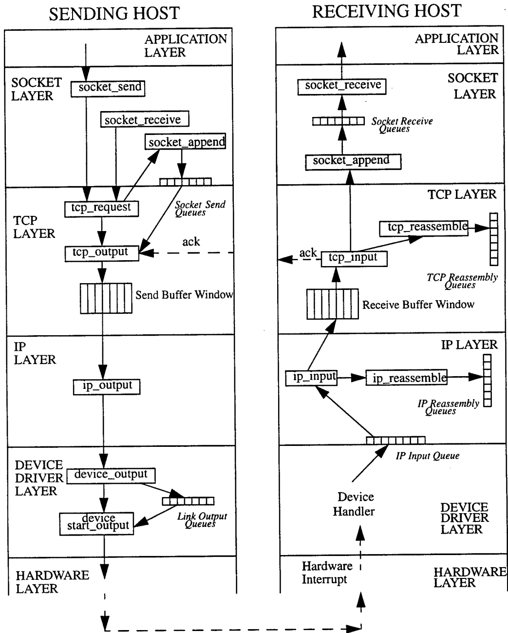
Figure 2: Data Flow
