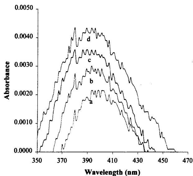
Figure 11. UV-Vis Absorbance of Polydy6 Thin-Films [(a) 5 bilayers; (b) 10 bilayers; (c) 15 bilayers; (d) 20 bilayers].
