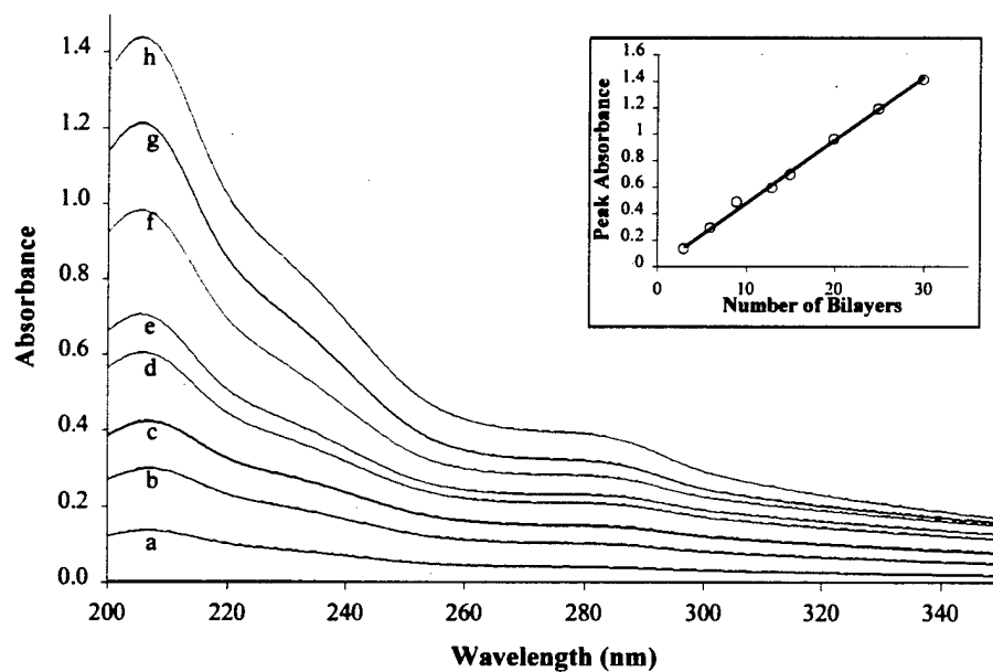
Figure 12. UV-Vis Absorbance of Polydy7 Thin-Films [(a) 3 Bilayers; (b) 6 Bilayers; (c) 9 Bilayers; (d) 13 Bilayers; (e) 15 Bilayers; (f) 20 Bilayers; (g) 25 Bilayers; (h) 30 Bilayers] with Inset Showing the Linear Relationship Between Absorbance at 208 nm and the Number of Bilayers Assembled.
