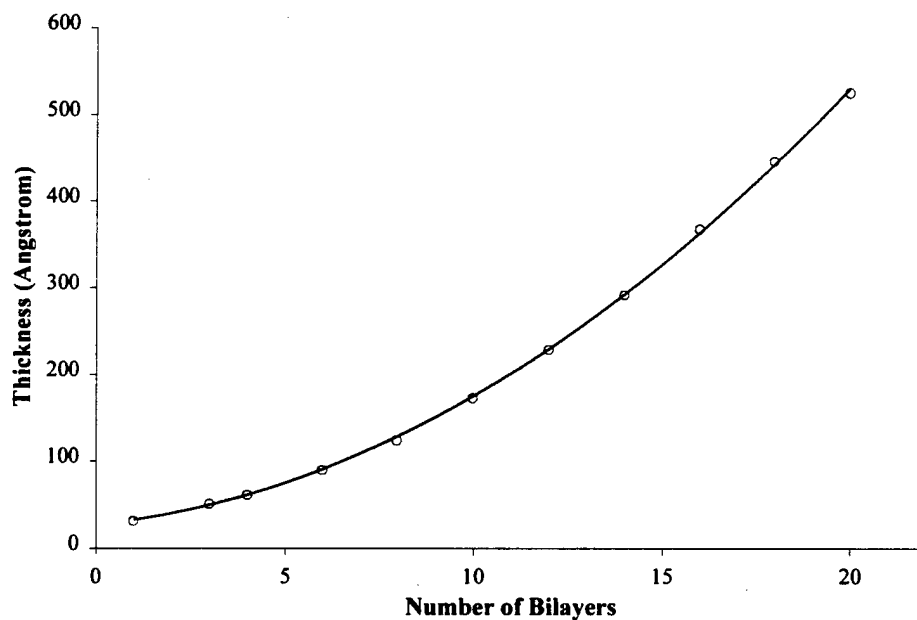
Figure 18. Polydye1/PDDA ISAM Film Thickness.
