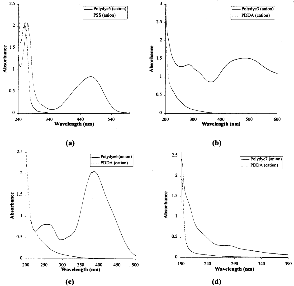
Figure 9. UV-Vis Spectra of (a) Polydye3; (b) Polydye5; (c) Polydye6; and (d) Polydye7 Aqueous Solutions.
