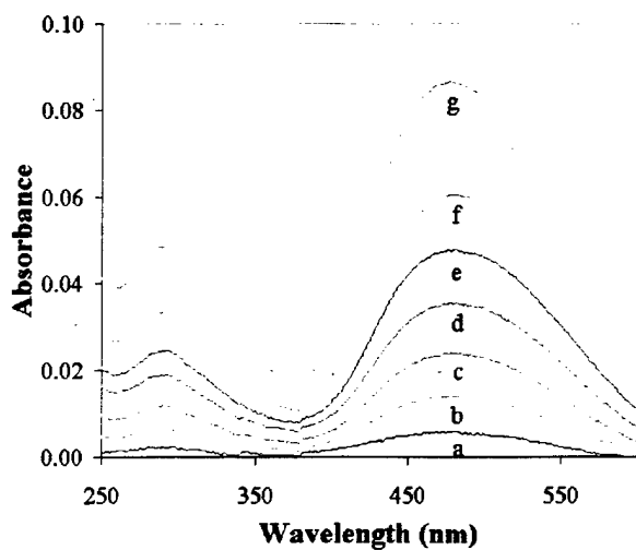
Figure 16. UV-Vis Absorbance of Polydye1 Thin-Films [(a) 2 Bilayers; (b) 4 Bilayers; (c) 6 Bilayers; (d) 8 Bilayers; (e) 10 Bilayers; (f) 12 Bilayers; (g) 16 Bilayers].
