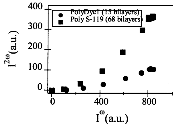
Figure 20. Comparison of SHG Signal for 15 Bilayer Polydye1 and 68 Bilayer Poly S-119 ISAM Films.
