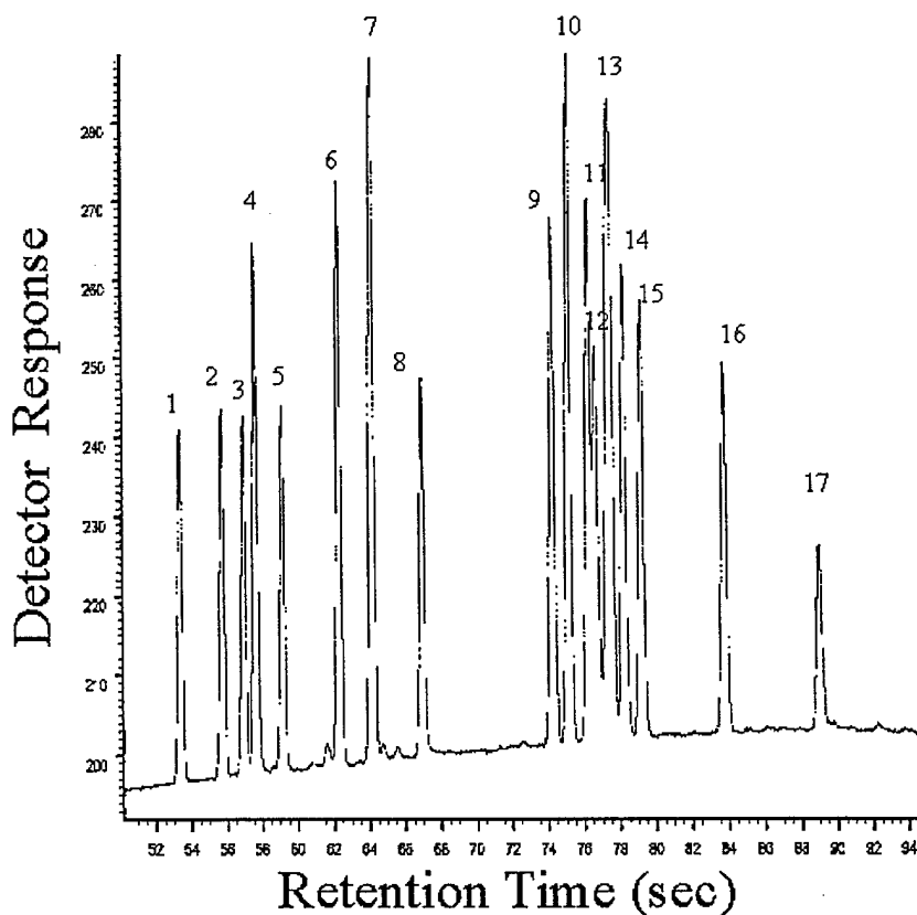
Figure 1. Flash™ GC separation of a sample containing a mixture of volatile and semi-volatile components with a wide-boiling range
