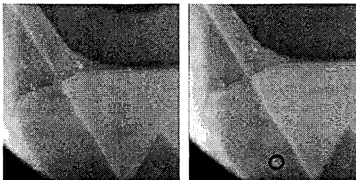
Figure 3. After pulsing for 500 ms with a +2.5 V pulse, a bright spot is seen to the left of the image, indicating the insertion of 2 . These images (R970617105 and R970617106) have overall heights of 20 Å and dimensions of 250 × 250 nm (300 mV, 100 pA).
