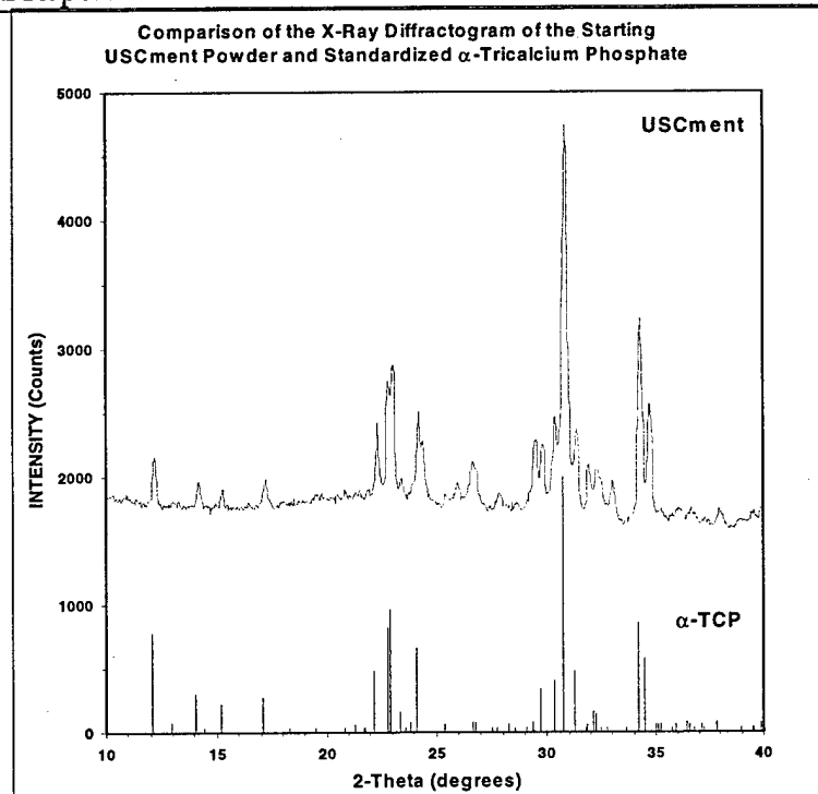
Figure 5. Powder X-ray Diffraction of USCment. X-ray diffraction pattern of USCment was obtained in the Department of Chemistry and Biochemistry, University of South Carolina by Drs. Claridge and Zur Loye using a Rigaku X-Ray Diffractometer. Note the similarity in the diffraction peaks of USCment and standardized \alpha -TCP.
