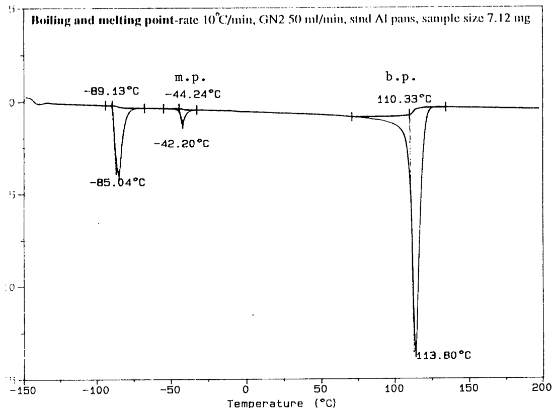
Figure 8 DSC Behavior of Quadricyclane
