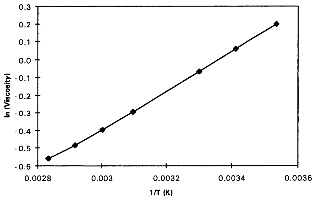
Figure 7 ln(Viscosity) versus 1/T
