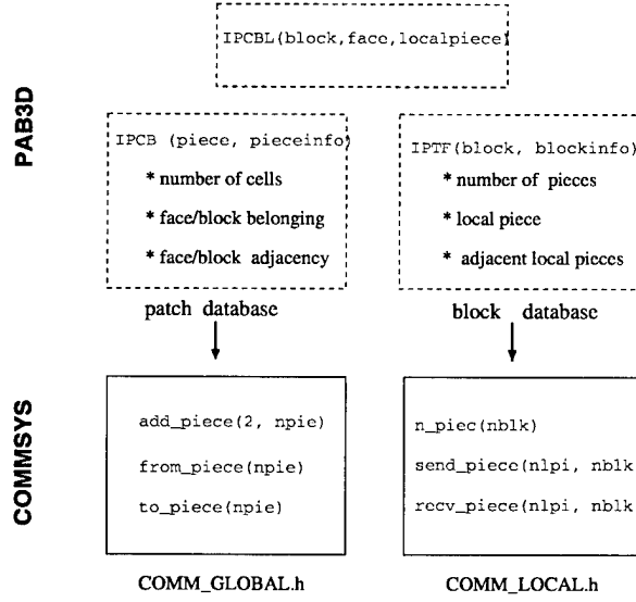
FIG. 5.6. Relation between the databases of PAB3D and those of COMMSYS
