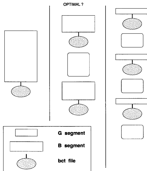
FIG. 6.1. Optimal segmentation
