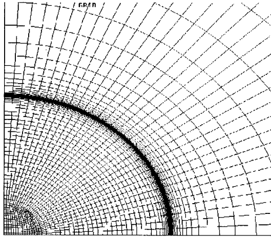
FIG. 2.3. A cross section of the prototype problem
