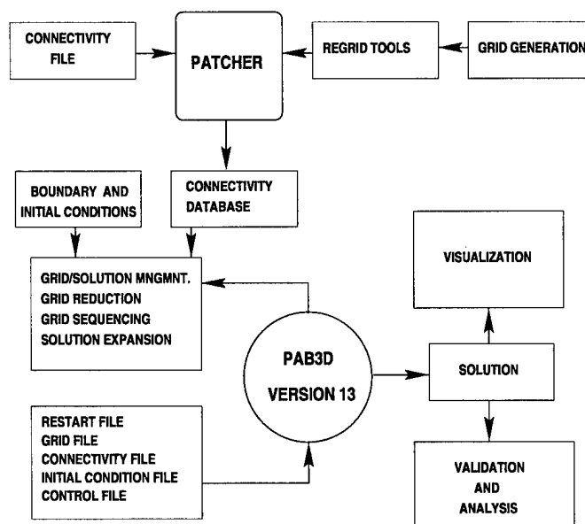
FIG. 2.1. Use of PAB3D, Version 13, and related programs and files
