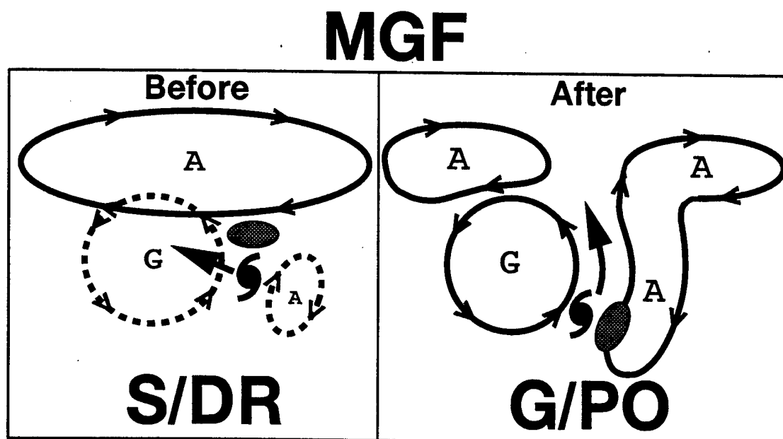
Figure 6. Conceptual model of Monsoon Gyre Formation (MGF). Solid streamlines indicate established features while dashed streamlines indicate a developing gyre and peripheral anticyclone. Arrows indicate TC motion. Shaded elliptical regions relative to the TC positions represent the isotach maximum. The TC typically undergoes a transition from S/DR to G/PO.
