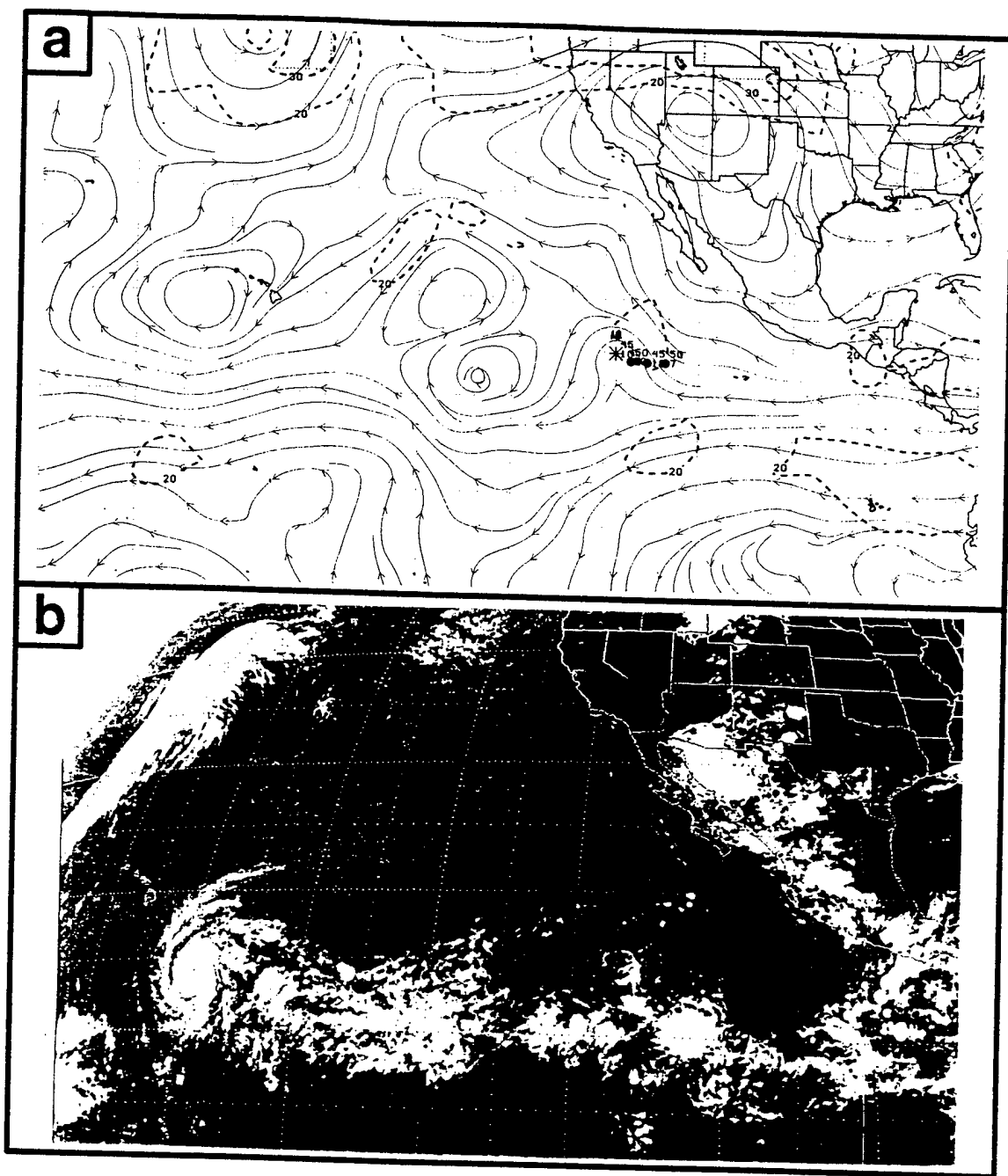
Figure 19. (a) NOGAPS 500-mb analysis as in Fig. 17, except at 12 UTC 17 August 1994. (b) GOES infrared imagery at 05 UTC 22 August 1994.
