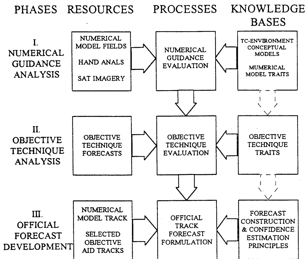
Figure 2. Flow chart of the three phases (left side) and components (top) in the Systematic Approach (from Carr and Elsberry 1994). This study will focus on the first phase only.
