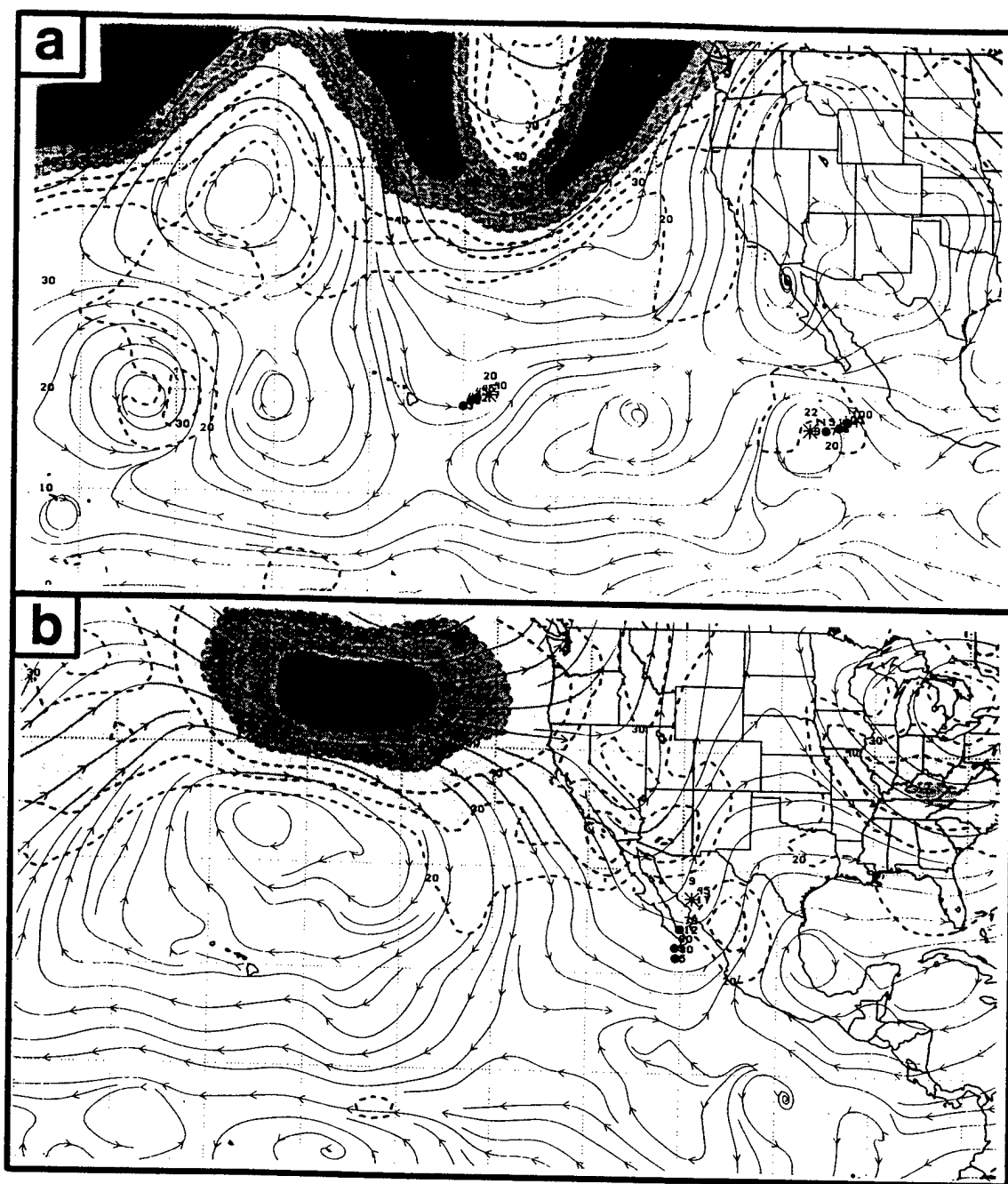
Figure 21. NOGAPS 500-mb analyses as in Fig. 17, except they illustrate S/MW cases at (a) 00 UTC 29 September 1992 (TS Roslyn is TC #20 near Hawaii; Hurricane Tina is TC #22 to the east) and (b) 12 UTC 14 September 1996 (TS Fausto).
