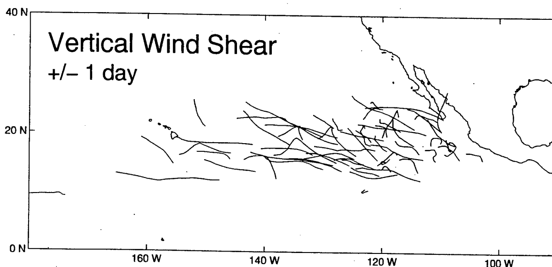
Figure 47. Tracks as in Fig. 1, except only when the TCs were undergoing the VWS transitional mechanism with up to a day before and after the process plotted. Circles at the ends of the tracks have been omitted in order to make the tracks more visible.
