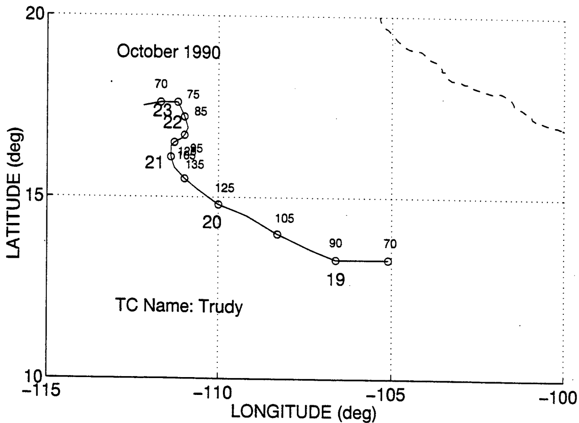
Figure 43. Best track, as in Fig. 34, except for Hurricane Trudy in October 1990.
