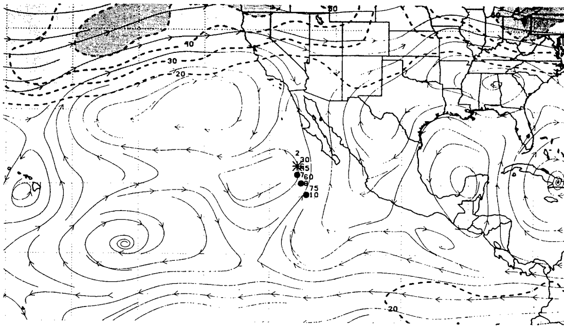
Figure 24. NOGAPS 500-mb analysis as in Fig. 17, except it illustrates a P/PO case at 12 UTC 7 June 1990 (TS Boris).
