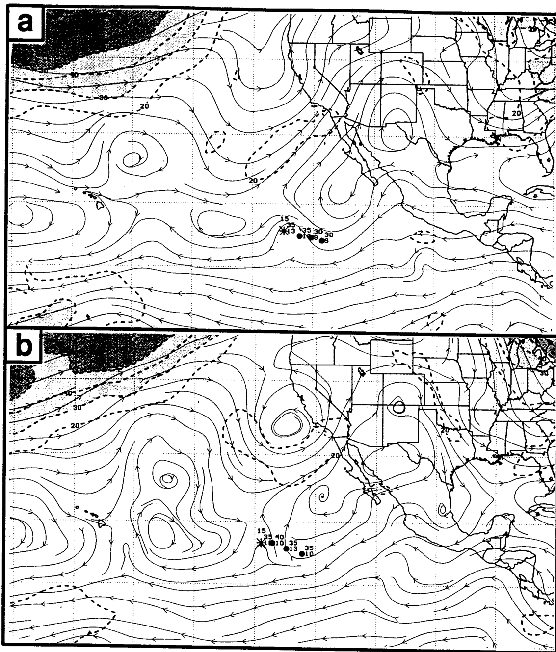
Figure 46. NOGAPS 500-mb analyses as in Fig. 17, except at 00 UTC (a) 18 and (b) 19 September 1994.
