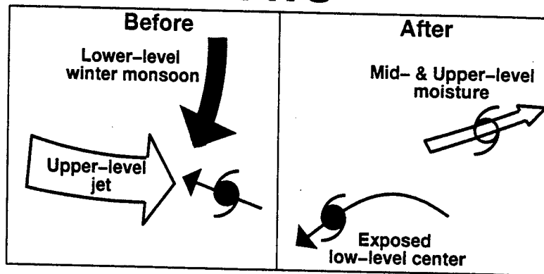
Figure 12. Conceptual model of Vertical Wind Shear (VWS). Upper-level southwesterlies advect the mid- and upper-level moisture northeastward while lower-level northeasterlies of the winter monsoon push the exposed low-level center of the TC to the southwest. Although the TC usually stays in S/DR during the entire time, the track exhibits a sudden turn.
