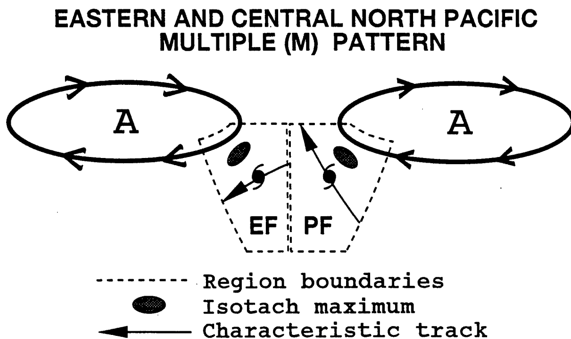
Figure 29. Conceptual model as in Fig. 16, except for Multiple (M) synoptic pattern and Equatorward Flow (EF) and Poleward Flow (PF) synoptic regions.
