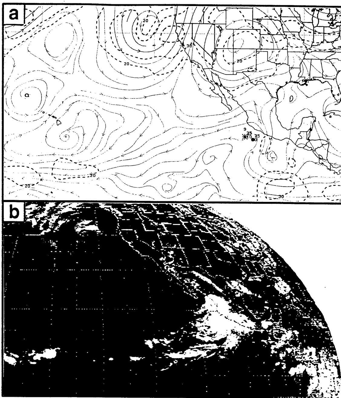
Figure 35. (a) NOGAPS 500-mb analysis as in Fig. 17, except at 12 UTC 1 September 1995. (b) GOES infrared imagery at 1130 UTC 1 September 1995.
