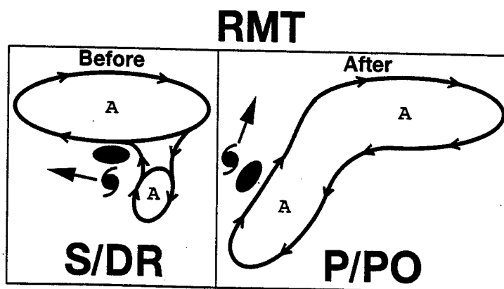
Figure 8. Conceptual model of Ridge Modification by a TC (RMT). A small peripheral anticyclone southeast of the TC grows, attaches to the STA, and modifies the STA. The TC typically undergoes a transition from S/DR to P/PO.
