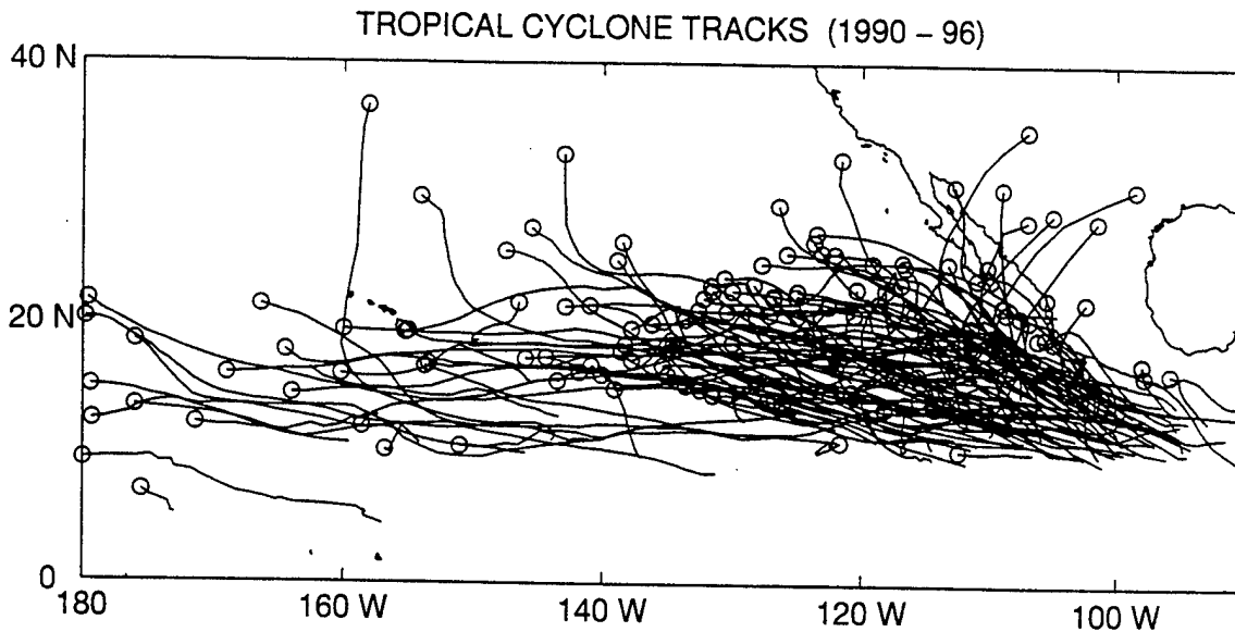
Figure 1. Summary of TC tracks from NHC and CPHC during 1990 - 96. The ending position is indicated with a circle.
