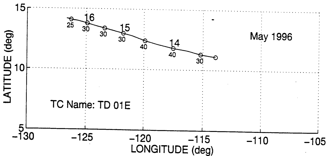
Figure 37. Best track, as in Fig. 34, except for TD 01E in May 1996.
