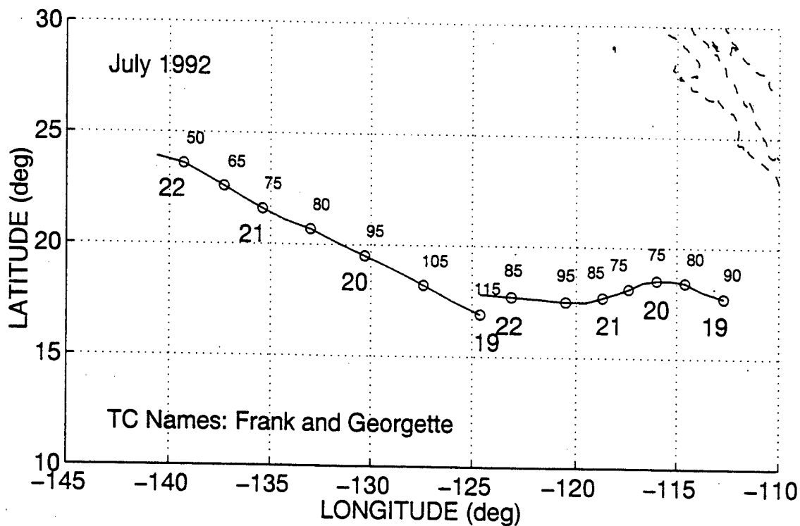
Figure 48. Best track, as in Fig. 34, except for Hurricanes Frank (west) and Georgette (east) in July 1992.
