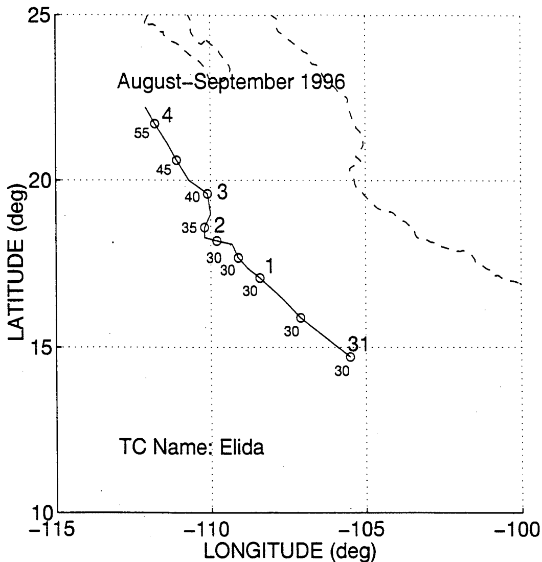
Figure 39. Best track, as in Fig. 34, except for TS Elida in August-September 1996.
