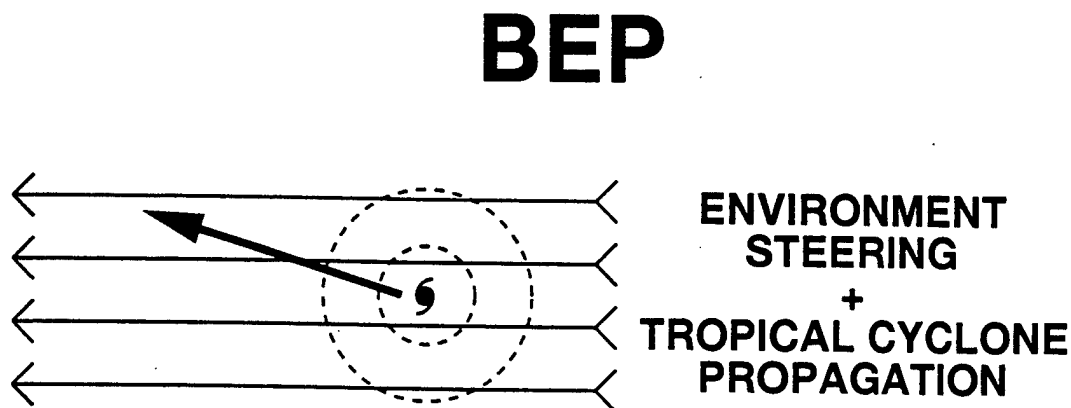
Figure 7. Conceptual model of Beta-Effect Propagation (BEP). In this case, the TC propagates toward the northwest within a background flow of easterlies.
