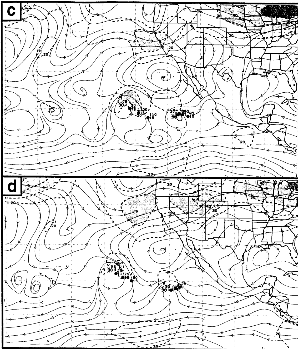
Figure 49. (continued) Like (a), except at 12 UTC (c) 20 and (d) 21 July 1992.
