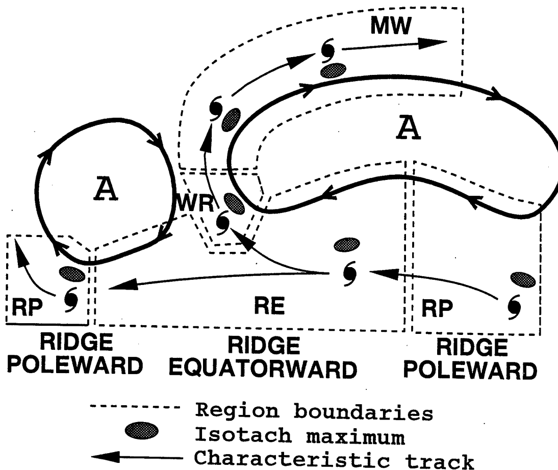
Figure 16. Conceptual model of Standard (S) synoptic pattern for the Eastern and Central North Pacific. Thick solid streamlines represent the 500-mb environmental flow after removal of the TC circulation. Light solid arrows illustrate characteristic tracks. Isotach maxima relative to the TC positions are indicated by shaded elliptical regions. Light dashed lines enclose the Ridge Poleward (RP), Ridge Equatorward (RE), Weakened Ridge (WR), and Midlatitude Westerlies (MW) synoptic regions.
