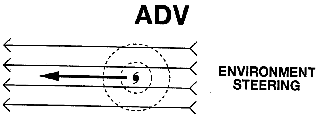
Figure 5. Conceptual model of Advection (ADV). The TC is simply advected along by the environment steering in that same direction.
