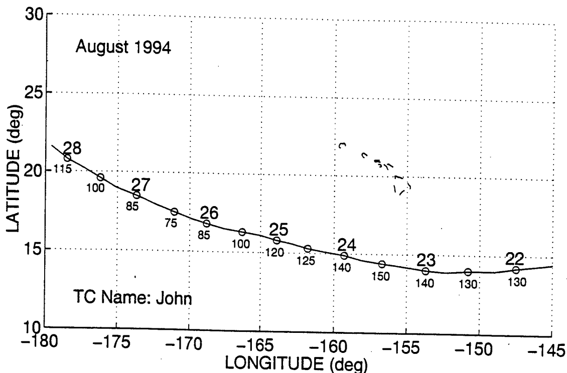
Figure 36. Best track, as in Fig. 34, except for Hurricane John in August 1994.
