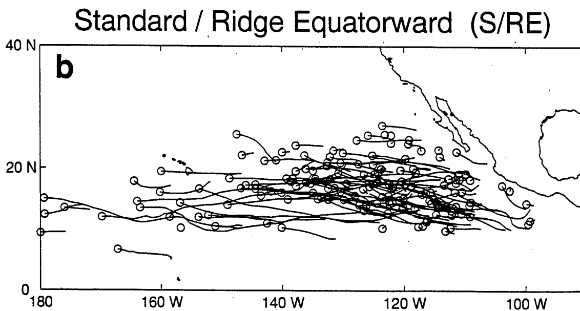
Figure 22. Tracks as in Fig. 1, except only while the TCs were in the Standard (S) synoptic pattern and (a) Ridge Poleward (RP) or (b) Ridge Equatorward (RE) synoptic regions.
