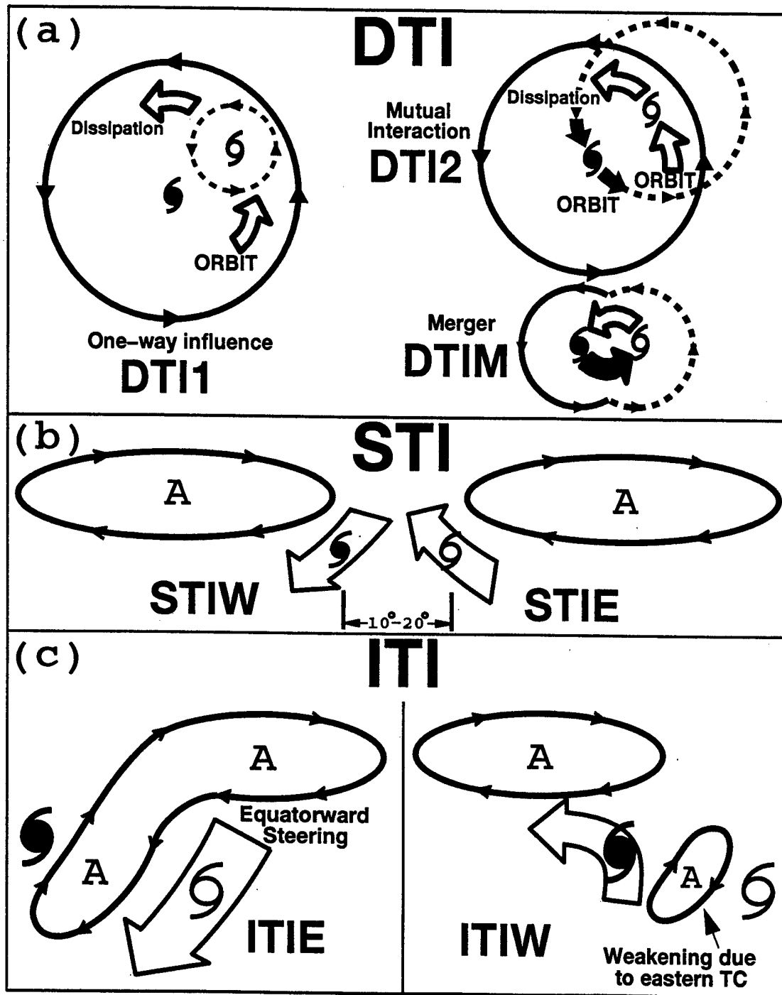
Figure 11. Conceptual models of TC Interactions. (a) Three types of Direct TC Interactions (DTI) exist owing to the difference in relative sizes of the TCs. (b) Semi-direct TC Interactions (STI) involve a Western (Eastern) TC undergoing STIW (STIE), but not necessarily simultaneously. (c) Two types of Indirect TC Interactions can occur depending upon the size and strength of the TCs.
