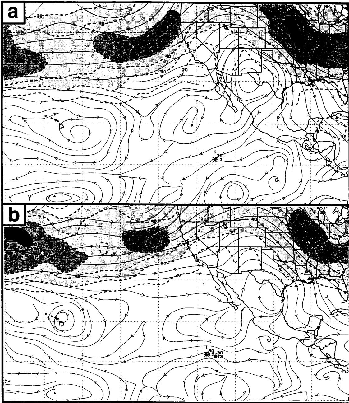
Figure 38. NOGAPS 500-mb analyses as in Fig. 17, except at (a) 12 UTC 13 May and (b) 00 UTC 14 May 1996.
