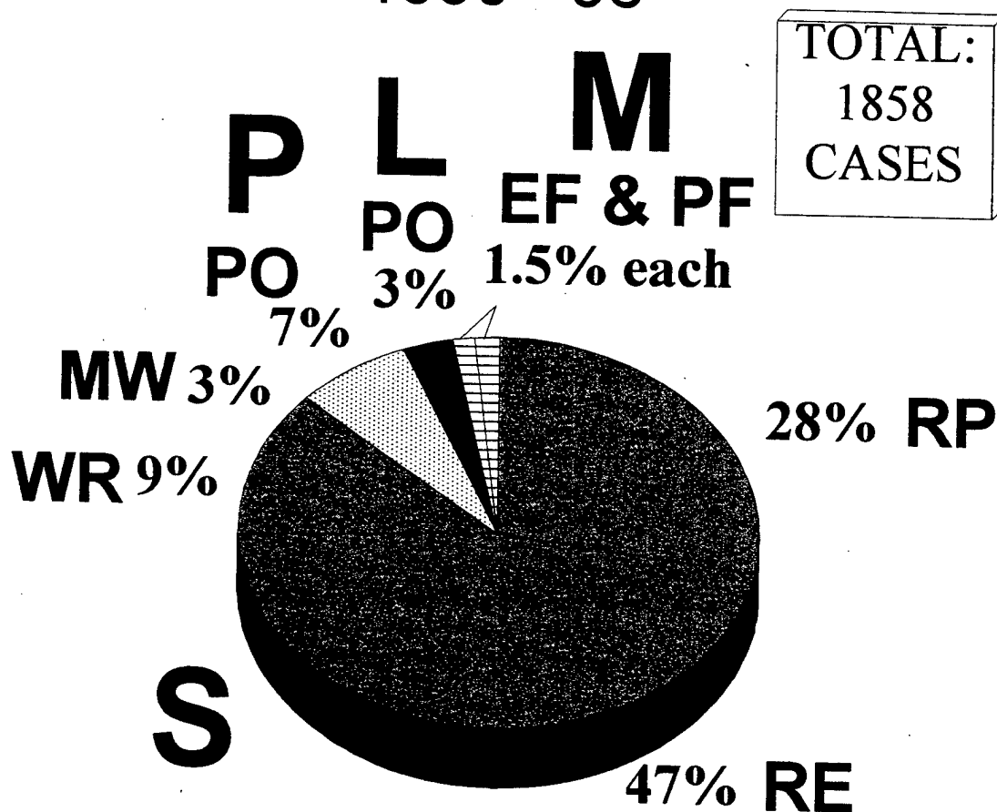
Figure 32. Climatology (percent) of synoptic pattern/regions in the ECPac environment structure for 1858 cases during 1990-96, with patterns separated by shading: S (grey), P (speckled), L (black), and M (lines).
