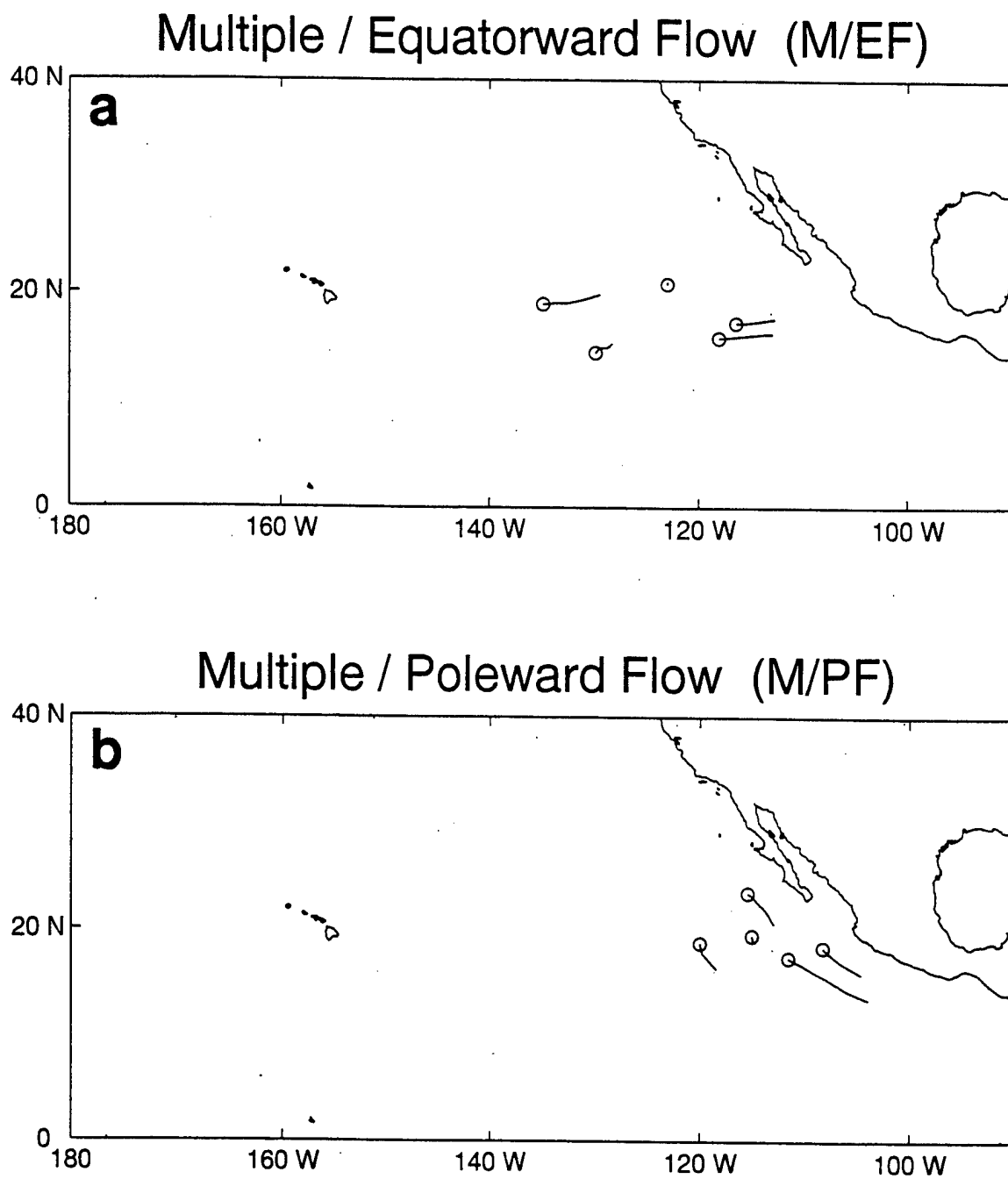
Figure 31. Tracks as in Fig. 1, except only while the TCs were in the Multiple (M) pattern and (a) Equatorward Flow (EF) or (b) Poleward Flow (PF) regions.
