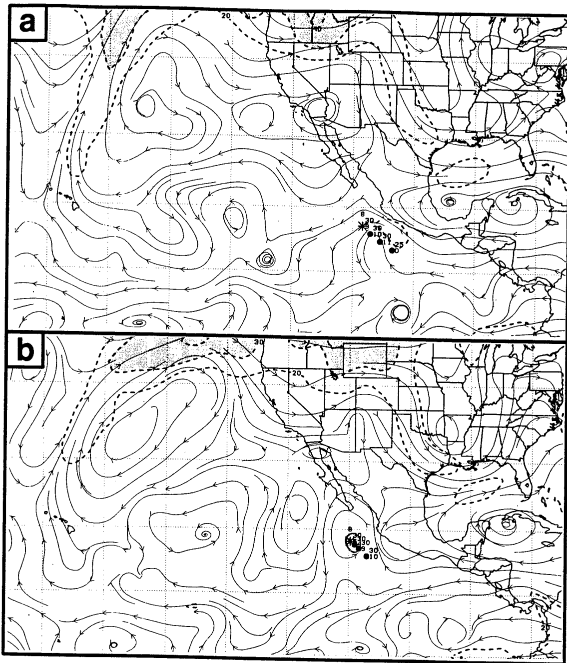
Figure 40. NOGAPS 500-mb analyses as in Fig. 17, except at 00 UTC (a) 1 and (b) 2 May 1996.
