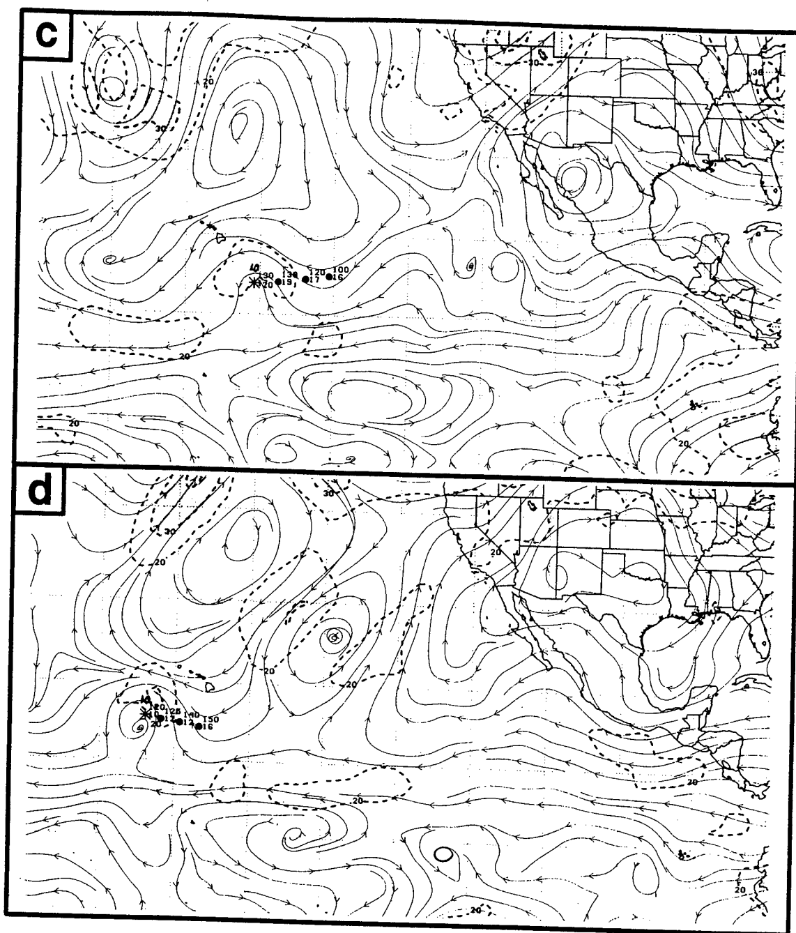
Figure 19. (continued) NOGAPS 500-mb analyses at (c) 12 UTC 22 August and (d) 00 UTC 25 August 1994.
