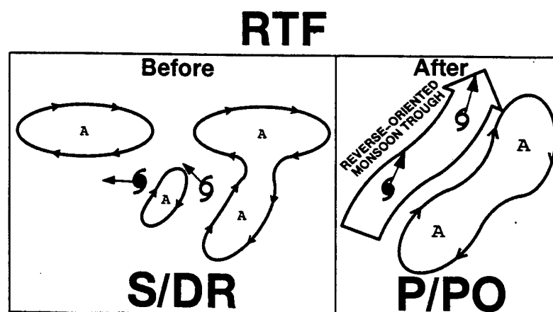
Figure 9. Conceptual model of Reverse Trough Formation (RTF). The peripheral anticyclones of more than one TC grow together, with the eastern anticyclone usually more dominant. The TCs typically undergo a transition from S/DR to P/PO within 24h of each other.
