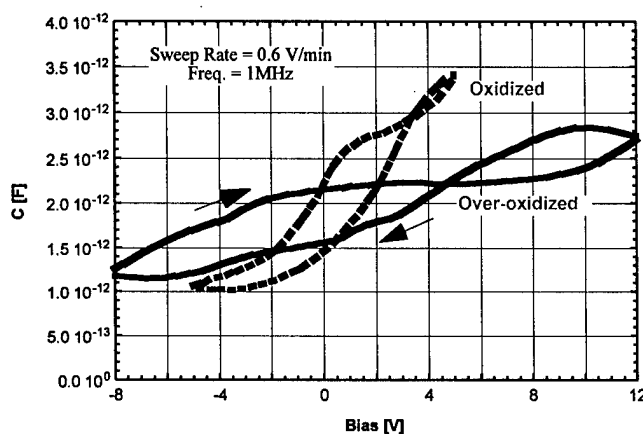
Figure 8. High frequency C - V curves for native oxide GaAs/ \text{Al}_2\text{O}_3 /Au MOS diodes
