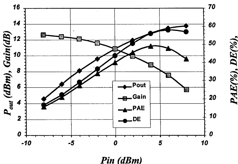
Figure 6: RF power and efficiency data for a 100\mu\text{m} wide GOIFET biased at 4.0 V drain bias. The data is taken at 3.0 GHz with single harmonic tuning in class AB mode.
