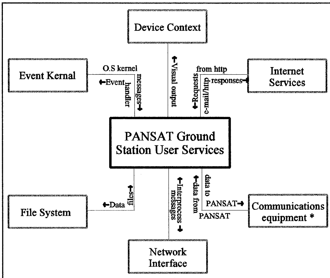
Figure 6 - Ground Station User Services Context Diagram
