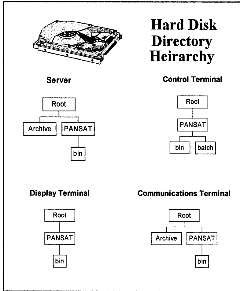
Figure 11 - Ground Station Initialization Directory Structure
