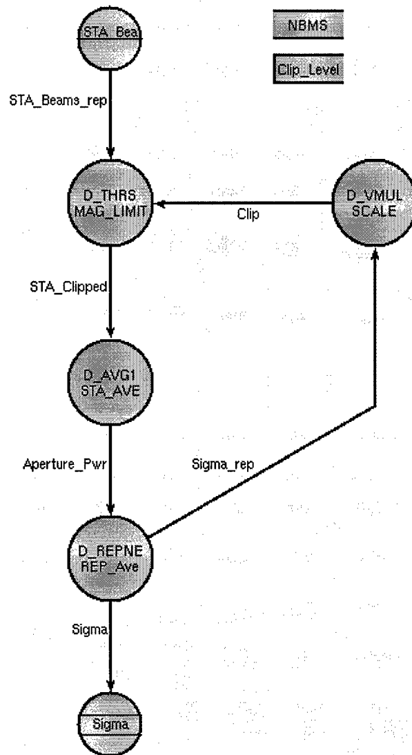
Figure 4. Normalizer Processing
