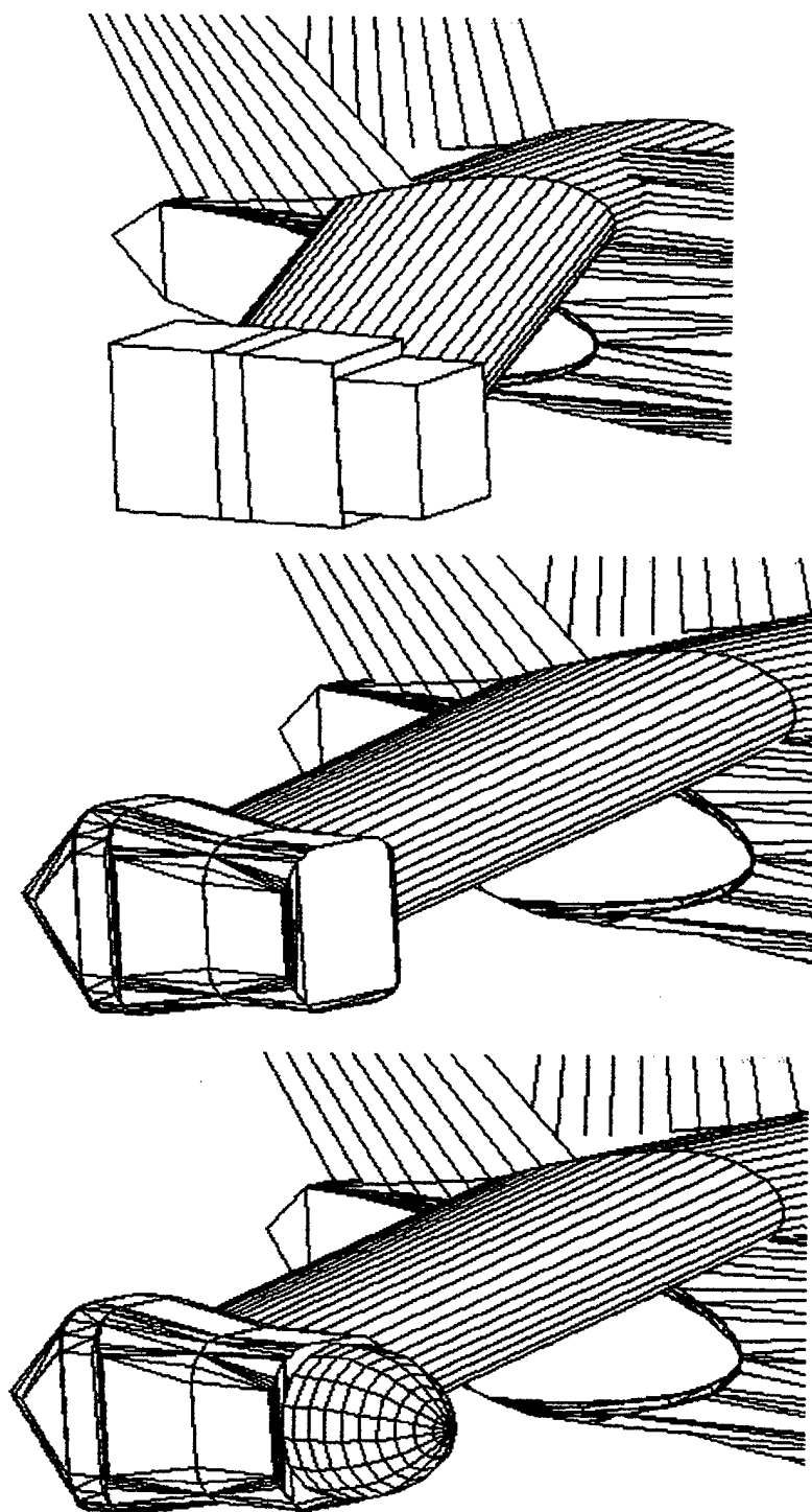
Figure 6.2 Construction of Wing Tip Nacelle
