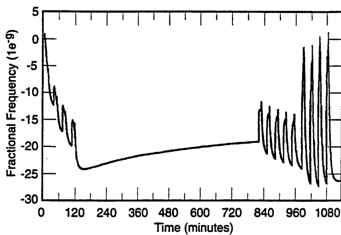
Fig. 11. Total dose sensitivity of SN1489 resonator (exposures: 3 x 20K, 5 x 40K, 4 x 160K)
