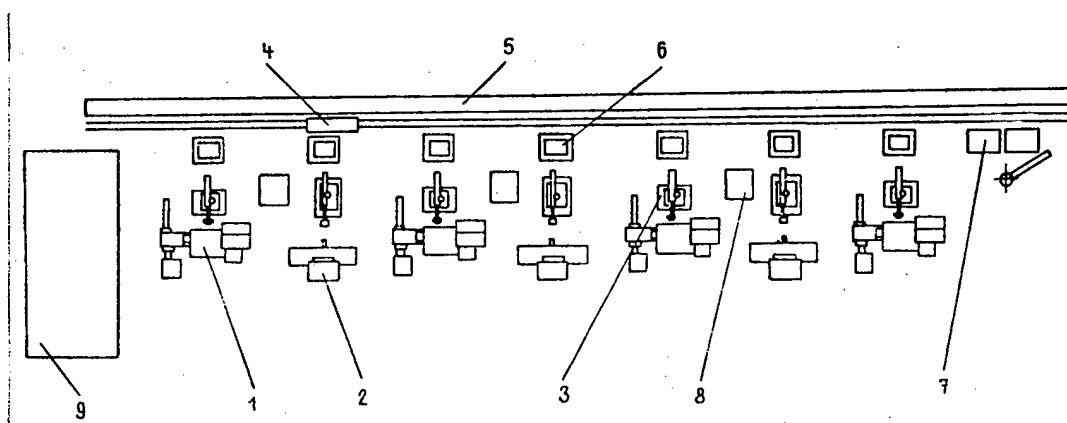
Figure 1. Layout of CAM System for Making the Light-Alloy End Shields of Electric Motors
