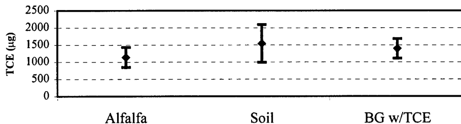
FIGURE 12. Recovered TCE (µg) from Air.
