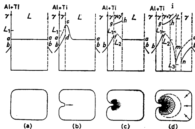
Figure 14. Schematic representation of process of ( \gamma + \gamma' ) eutectic formation (a) Liquid; (b) Beforehand stage; (c) Eutectic core formation; (d) Formation of eutectic cap and poor \gamma' zone
