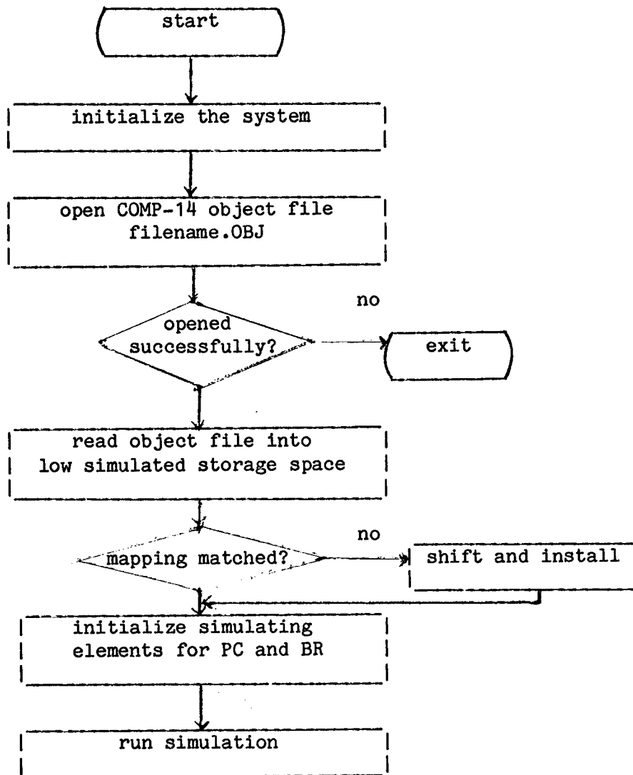
Figure 7. The CSIMUL Flowchart
