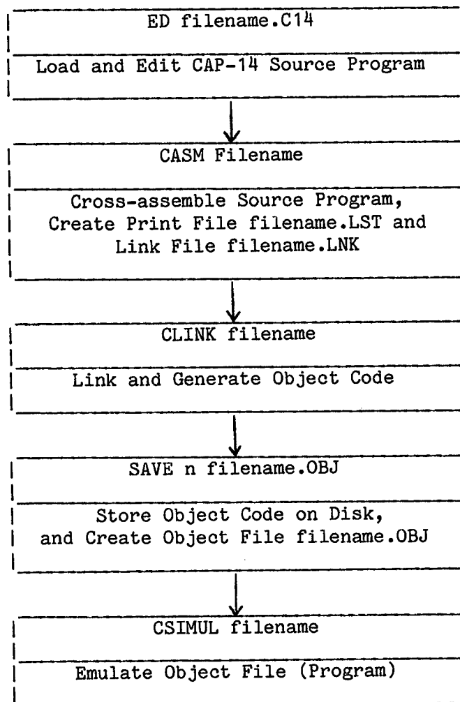
Figure 1. Cross Simulating Procedure of the CAP-14 Assembly Language
