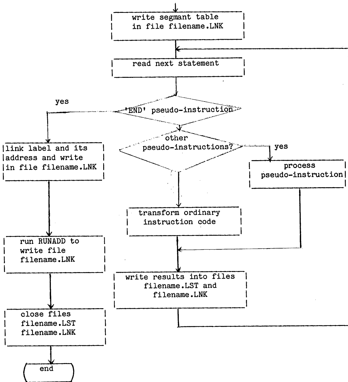
Figure 4. The CASM Flowchart
