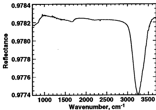
Figure 8. Calculated effect of 150 \text{ \AA} film of H_2O on 20K mirror reflectance.
