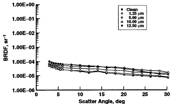
Figure 10. Mirror scatter due to argon films condensed at 16K and for 10.6 \mu m wavelength.
