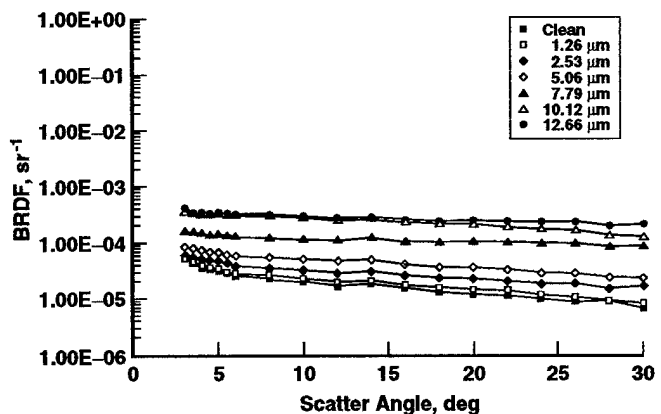
Figure 11. Mirror scatter due to oxygen films condensed at 16K and for 10.6 \mu m wavelength.
