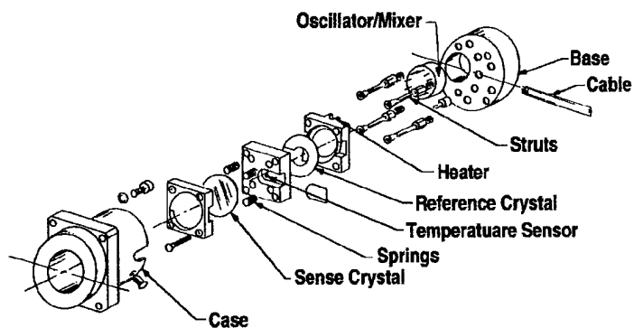
Figure 4. Mark 16 CQCM assembly diagram.
