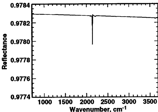
Figure 9. Calculated effect of 150 \text{ \AA} film of CO on 20K mirror reflectance.
