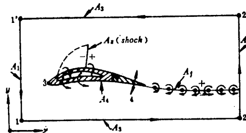
Figure 1. Unsteady Flow Over an Oscillating Airfoil
