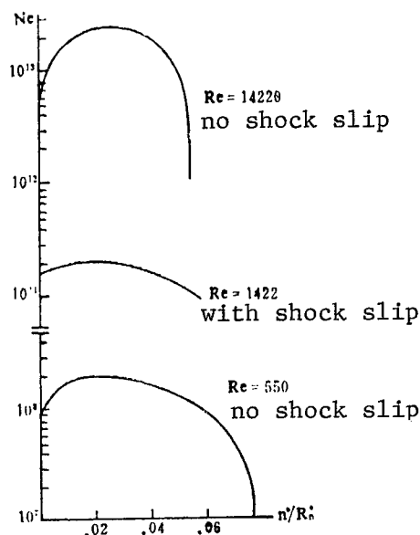
Figure 2. Electron Density Distribution at the Stagnation Point
