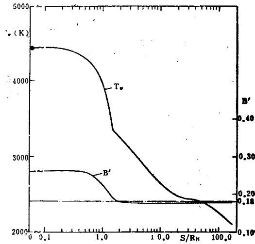
Figure 4. Variation of Wall Temperature and Mass Transfer Parameter Along the Surface — this paper; • Ref. [14]
