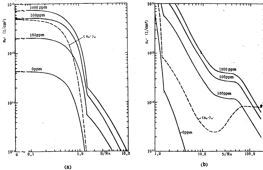
Figure 5. Variation of Electron Density Along the Surface --- value at the outer edge of boundary layer; • value at the outer edge given in Ref. [14]
