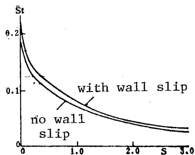
Figure 9. Distribution of Stanton Number Re = 2615 ; R_n = 1.22 m; U_\infty = 7.62 km/sec; T_w = 1000 K; T_\infty = 180.9 K
