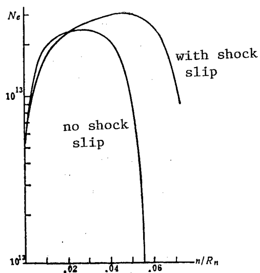
Figure 8. Distribution of Electron Density at the Stagnation Point U_\infty = 7.65 km/sec; Re = 14220 ; half cone angle = 30^\circ
