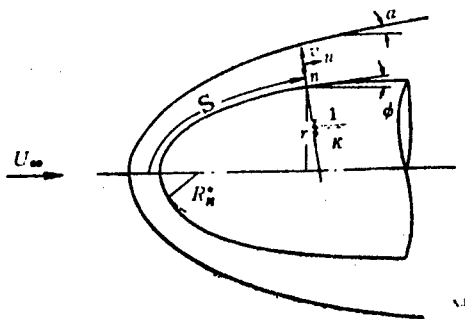
Figure 1. Surface Coordinate System
