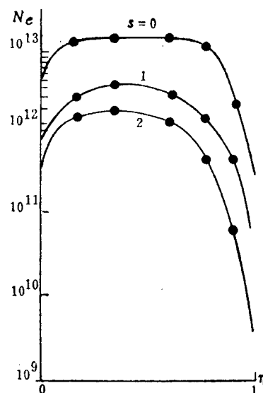
Figure 7. Distribution of Electron Density Re = 14220 ; M_\infty = 24.6 ; no slip; half cone angle = 10^\circ
