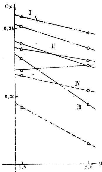
Figure 2. Variations of Drag Coefficients With Mach Number for Four Different Afterbodies
