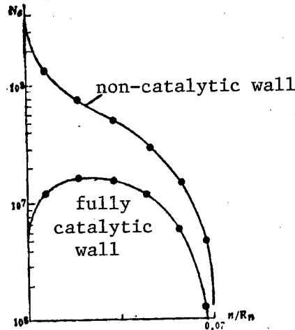
Figure 10. Distribution of Electron Density
