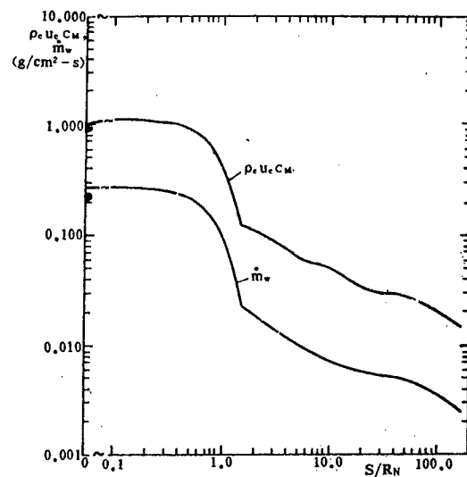
Figure 3. Variation of Ablation Rate and Mass Transfer Coefficient Along the Surface — this paper; • Ref. [14]
