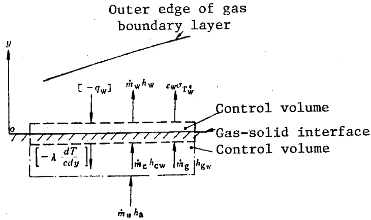
Figure 2. Conservation of Energy at the Gas-Solid Interface
