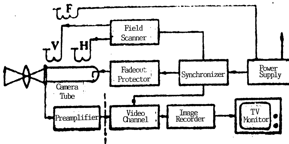
Figure 1. Basic schematics of the closed-circuit television system.
