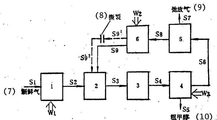
Figure 1. Flowsheet Diagram of Methanol Synthesis Process
