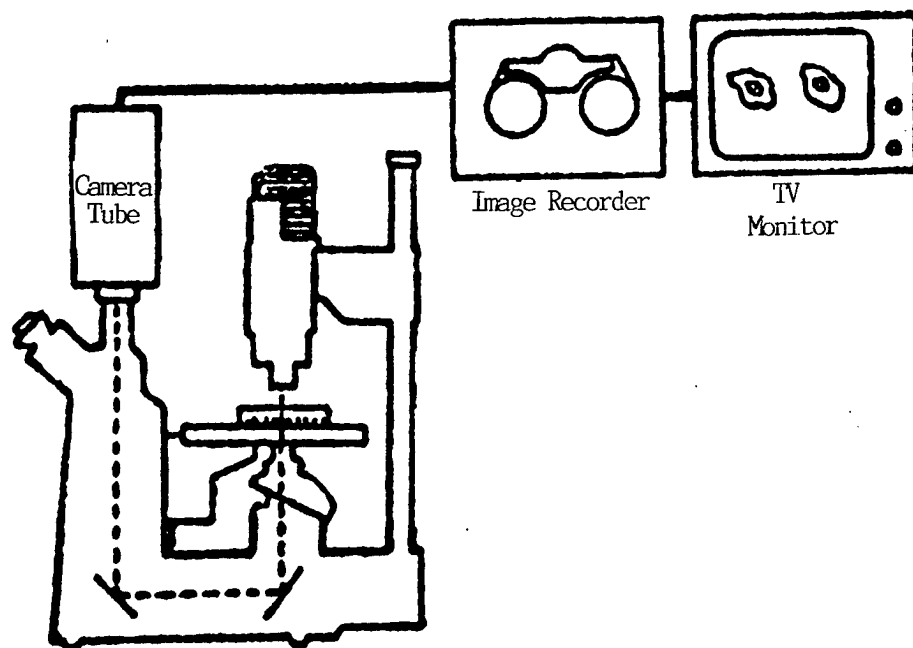
Figure 2. Setup for experiment observing and recording the microinjection of cells.
