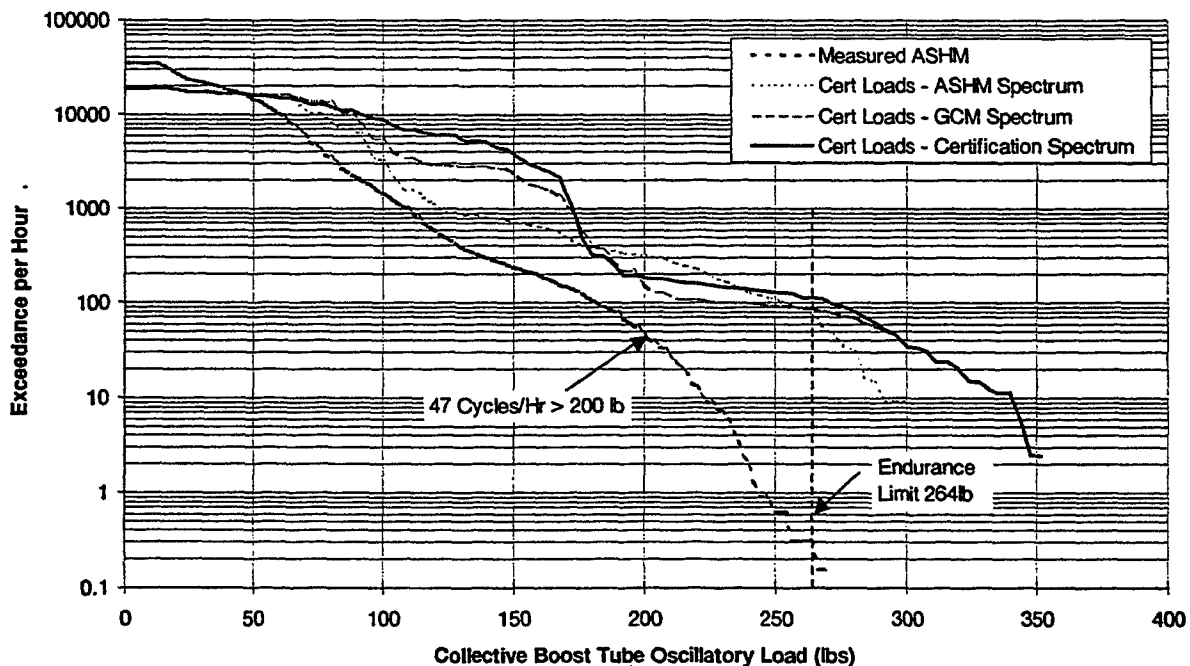
Figure 6.1 Collective Boost Tube Load Comparison
