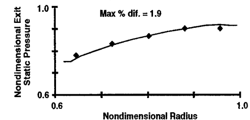
Fig. 15. Clean Inlet, exit static pressure on the 100-percent speedline.
