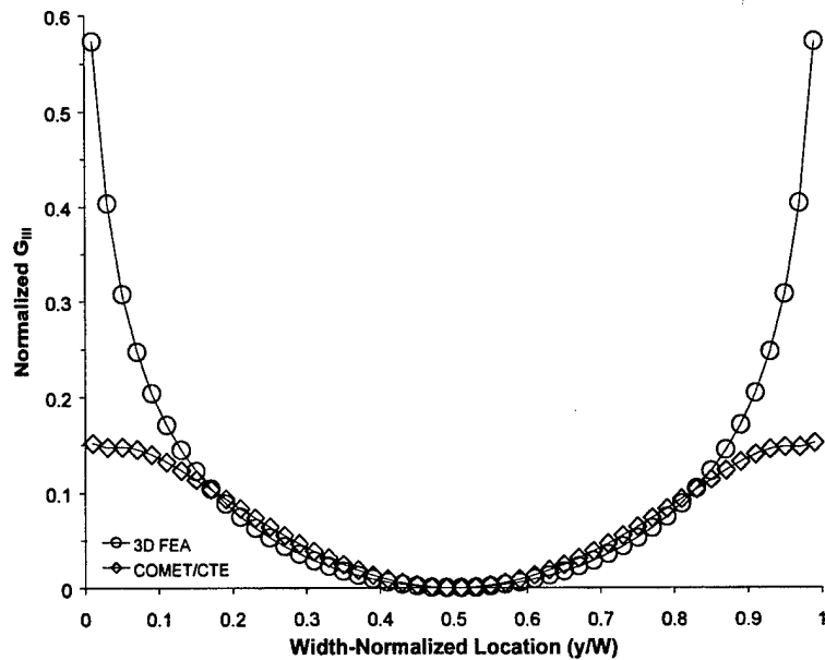
FIGURE 11b. COMPARISON OF CTE AND THREE-DIMENSIONAL FE PREDICTIONS OF G_{III} FOR M=0 LOADING
