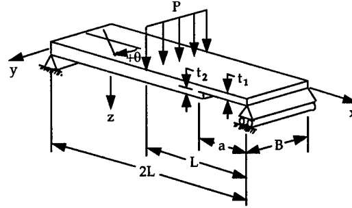
FIGURE 14. THE SINGLE LEG BENDING TEST
