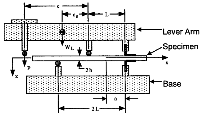
FIGURE 15. THE MIXED-MODE BENDING TEST
