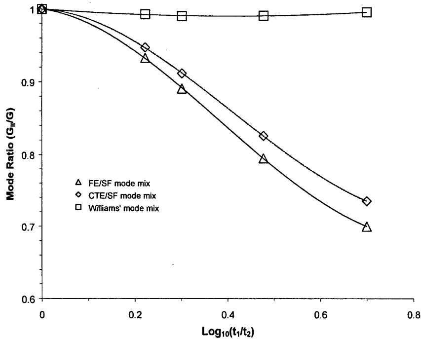
FIGURE 19b. MODE MIX VERSUS THICKNESS RATIO FOR THE UENF TEST, L = 2a , a/t = 6.94
