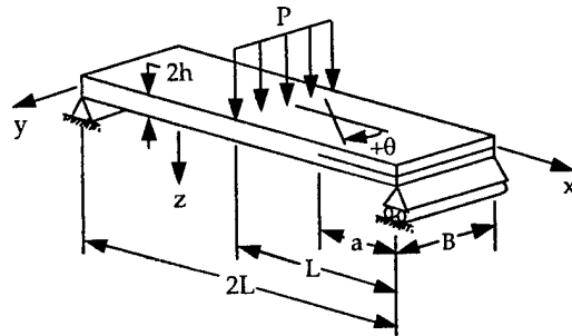
FIGURE 13. THE END-NOTCHED FLEXURE TEST
