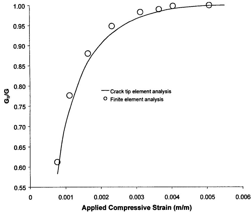
FIGURE 4b. COMPARISON OF MODE RATIO FOR A [0_2/90/0_2]_{3S} LAMINATE
