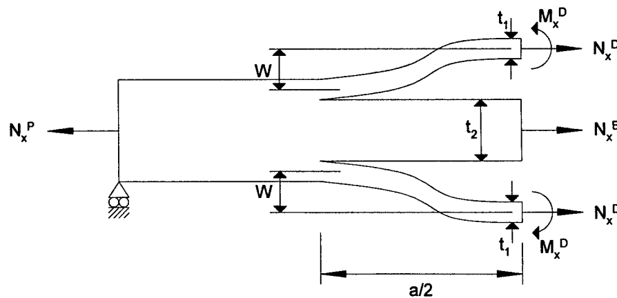
FIGURE 3a. POST-BUCKLED CONFIGURATION
