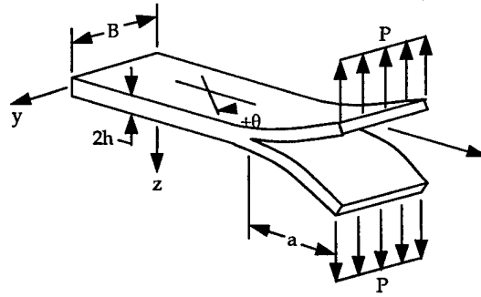
FIGURE 12. THE DOUBLE CANTILEVER BEAM TEST
