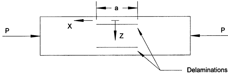
FIGURE 2. CROSS-SECTIONAL VIEW OF LAMINATE CONTAINING TWO SYMMETRICALLY LOCATED DELAMINATIONS THAT IS SUBJECTED TO COMPRESSIVE LOADING
