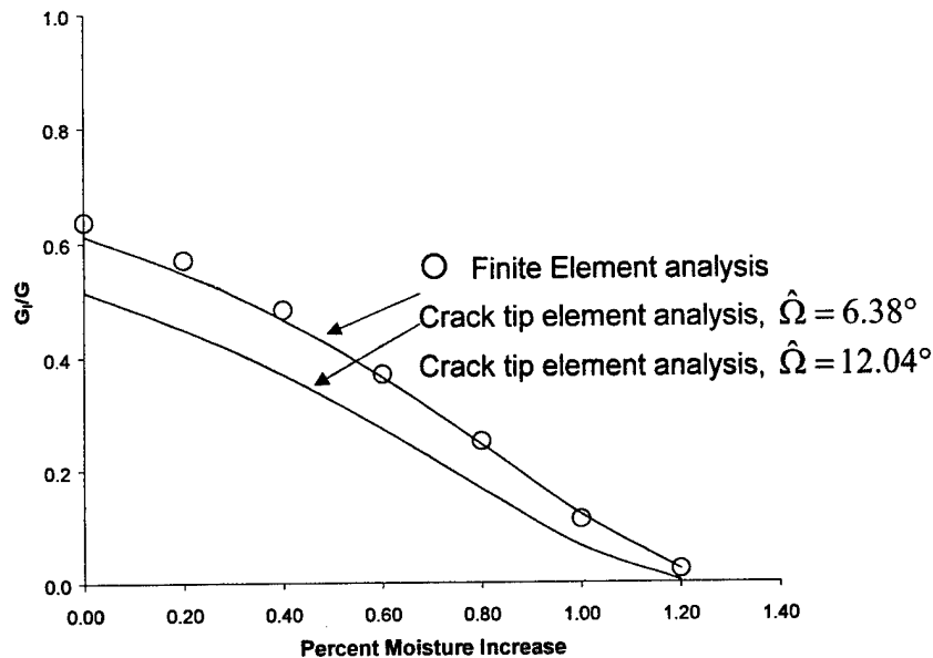
FIGURE 7. MODE RATIO VERSUS HYGROSCOPIC LOADING FOR A [0/\pm 35/90]_s T300/5208 LAMINATE WITH EDGE DELAMINATIONS AT BOTH -35/90 INTERFACES
