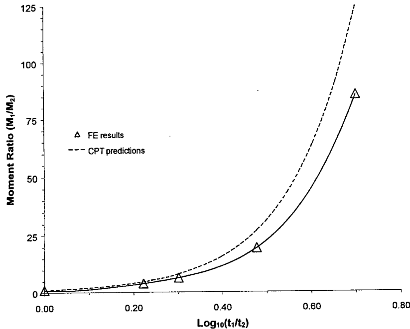
FIGURE 19a. MOMENT RATIO VERSUS THICKNESS RATIO FOR THE UENF TEST, L = 2a , a/t = 6.94
