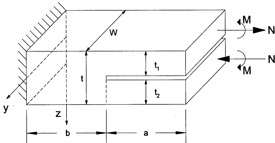
FIGURE 8. THREE-DIMENSIONAL PROBLEM AND LOADING
