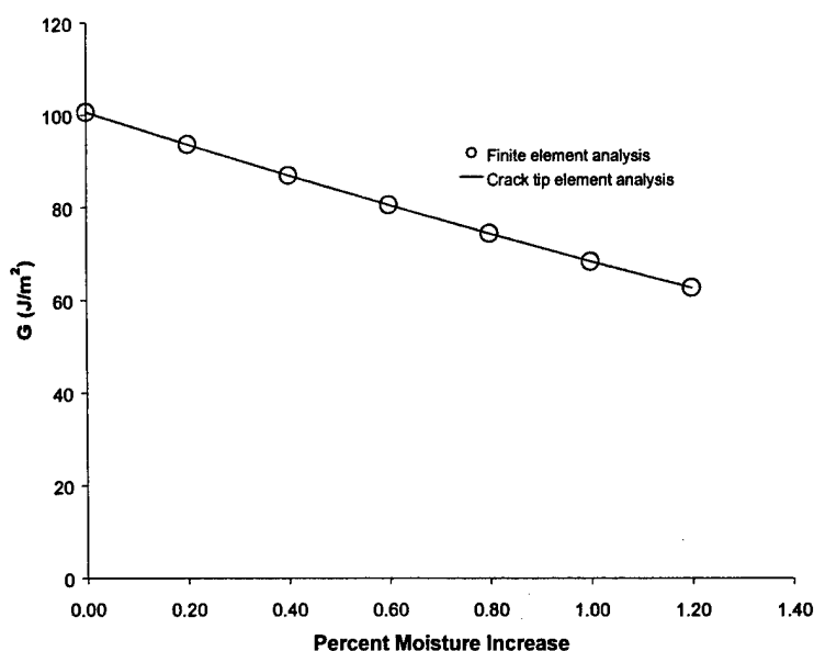
FIGURE 6. ERR VERSUS HYGROSCOPIC LOADING FOR A [45/0/-45/90]_s T300/5208 LAMINATE WITH EDGE DELAMINATIONS AT BOTH -45/90 INTERFACES
