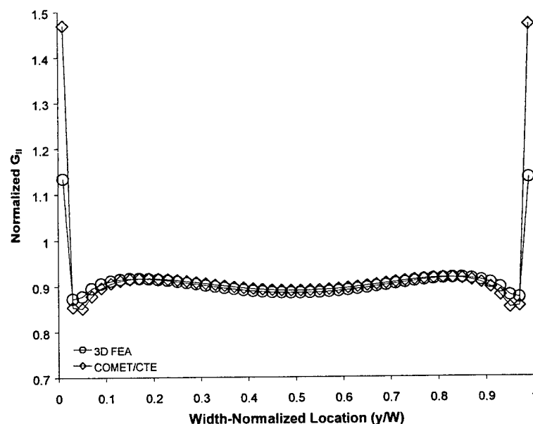
FIGURE 11a. COMPARISON OF CTE AND THREE-DIMENSIONAL FE PREDICTIONS OF G_{II} FOR M=0 LOADING
