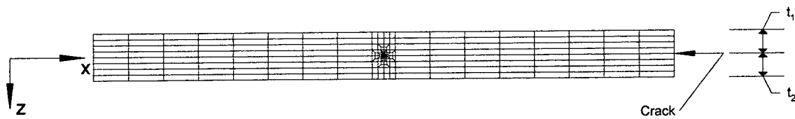
FIGURE 9c. FINITE ELEMENT MESH IN THE X-Z PLANE
