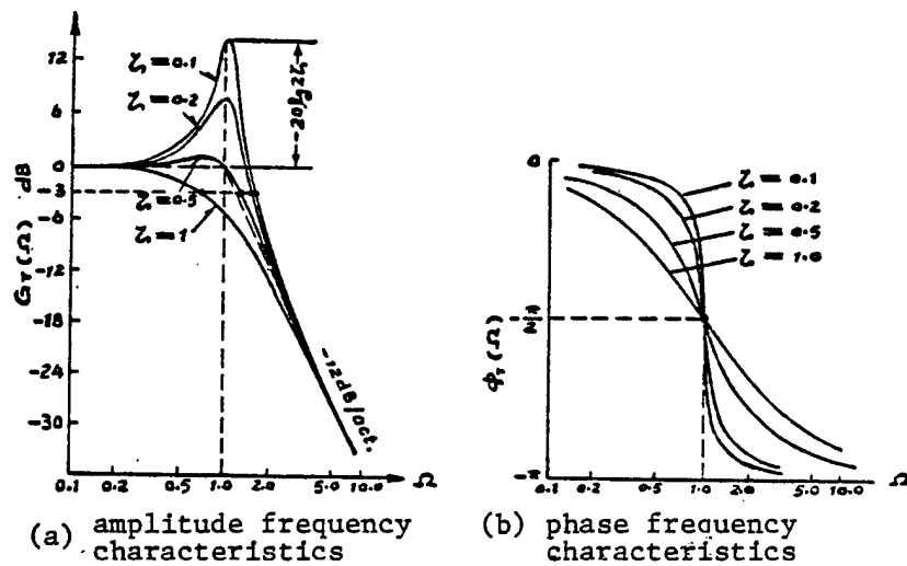
Figure 10. Frequency Characteristics of Variable Equalization Circuits
