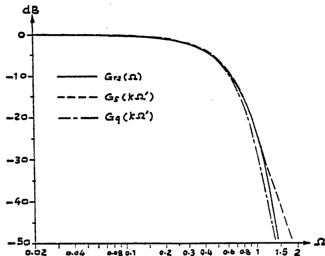
Figure 7. Approximation Conditions for 5th and 9th Order Gaussian Filters to the Gaussian Filter Required for Implementation
