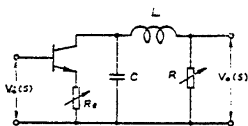
Figure 9. Structure of a Variable Equalization Circuit
