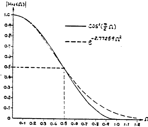
Figure 5. The Approximation of \exp(-2.77259\Omega^2) for H_{r2}(\Omega)
