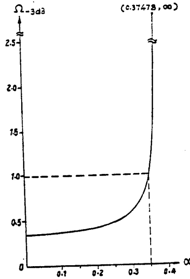
Figure 8. The Relation Between \Omega_{-3dB} and \alpha
