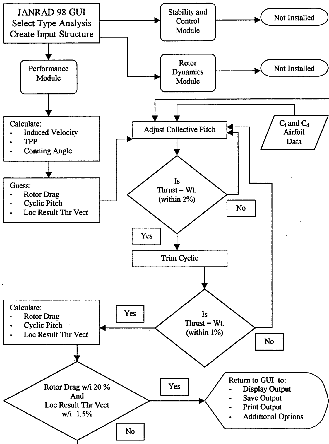
Figure 5. JANRAD Computation Flow Chart .
