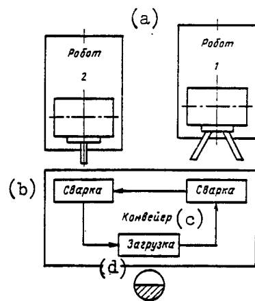
Fig. 2. Automatic line for assembly-welding of recess of cover of a tool box
