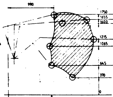
IRB 60/2: range of motions
