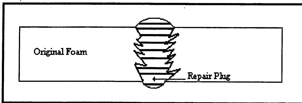
Figure 41. Sketch of a repaired foam block. Note that the new foam completely fills the cavity formed by the explosive blast. A cold joint is formed at the interface between the new and old foam.
