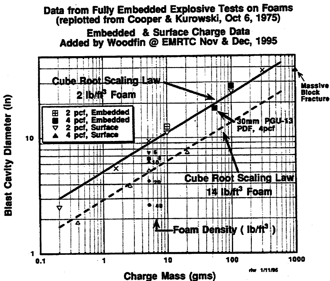
Figure 2. Blast cavity diameters from surface and embedded shots from Ref. [11] conducted by Cooper, Kurowski, and Woodfin. The solid line depicts the 2 lb/ft 3 foam while the dashed line depicts the 14 lb/ft 3 . The prediction of the foam densities (6, 8, 10, 20, and 40 lb/ft 3 ) were predicted by Cooper and Kurowski in 1976.
