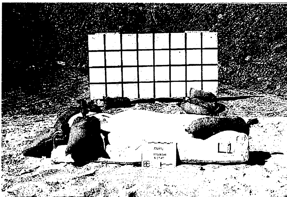
Figure 20. Set-up of Experiment L1. The sand bags kept the foam pad in contact with the ground during the blast. The grid in the background has an interline spacing of 1 foot.
