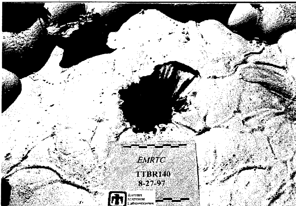
Figure 23. Exit cavity for Experiment L1, 6" thick, 10-gram charge
