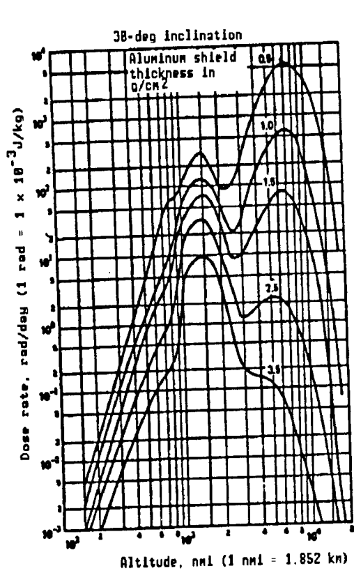
Figure 1. Trapped Proton Dose
