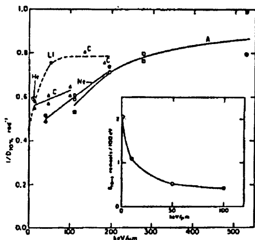
Figure 6. RBE vs. LET of V-79 Cell (Reference 5)
