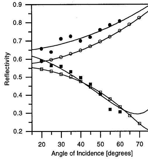
Figure 2: Reflectivity of Fe vs. angle of incidence at I = 10^{11} \text{ W/cm}^2 (open points) and 2 \times 10^{14} \text{ W/cm}^2 (filled points) for s-polarization (circles) and p-polarization (squares). The reflectivity of a density gradient calculated from the corresponding best fit results are shown with lines.
