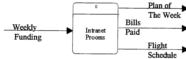
Figure 6.5 Grey Hole
