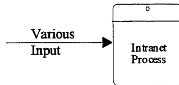
Figure 6.3 Black Hole
