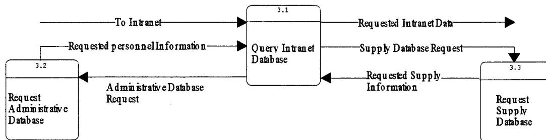
Figure 6.15 Level 1 DFD - Select Intranet Application
