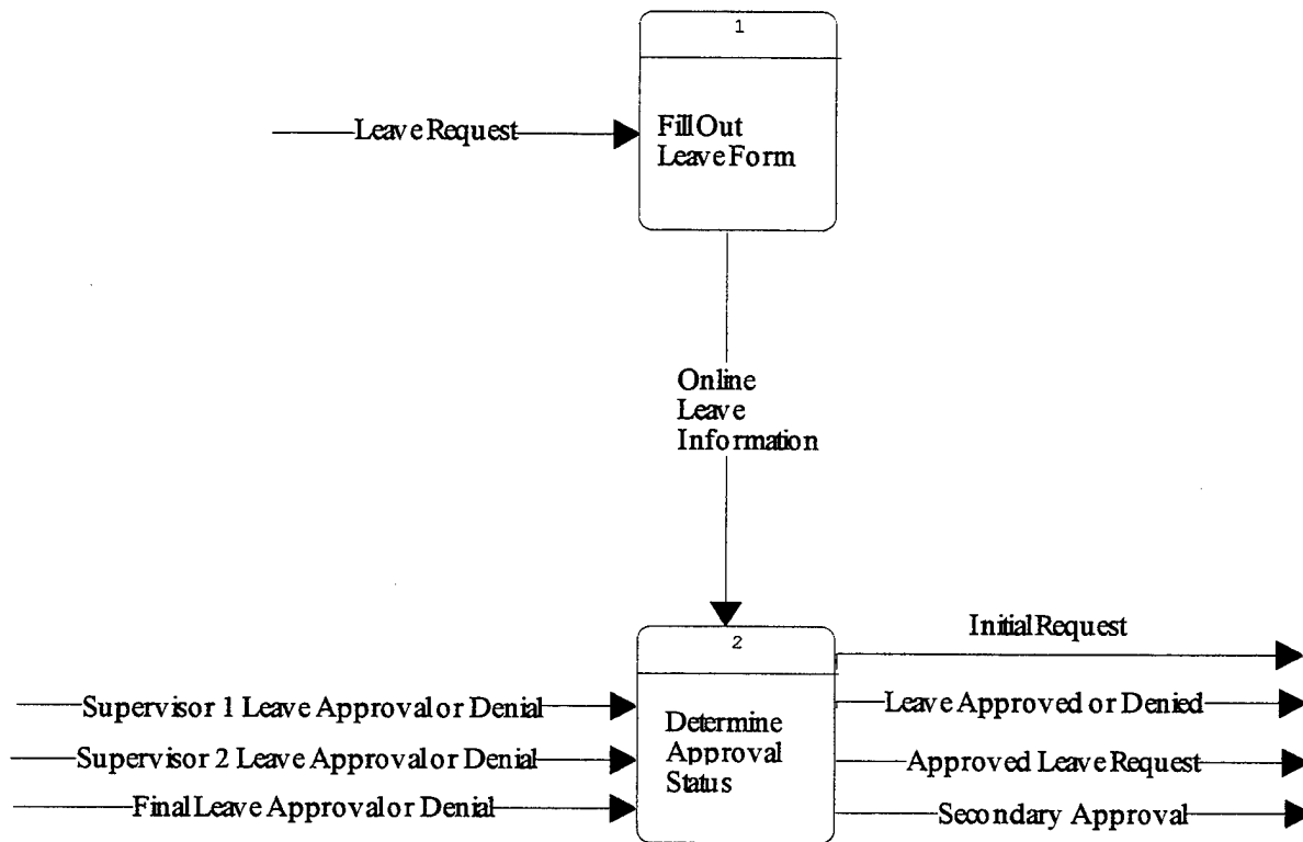
Figure 6.7 Level 1 DFD - Leave Request
