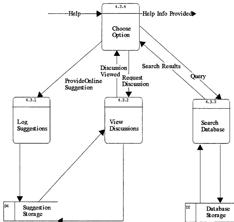
Figure 6.14 Level 2 DFD - Query Help Section
