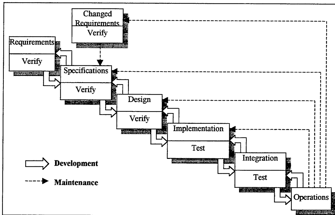
Figure 4.1 Waterfall Model, [Ref. 20, p. 46]
