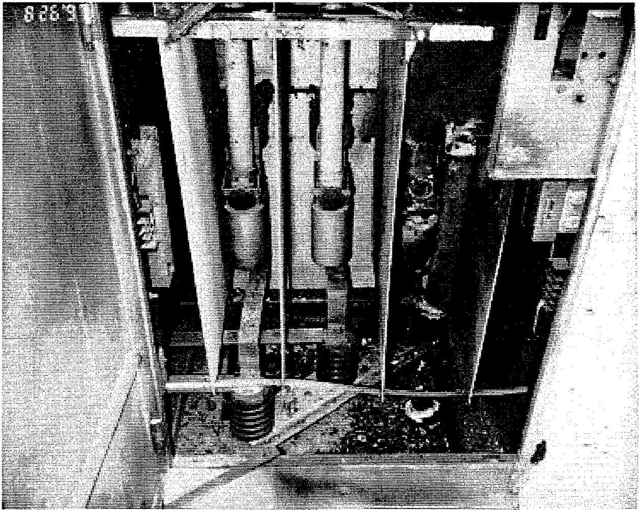
FIG. 17 EXPLODED L.I. SWITCH (right side) on PIER PROVIDING POWER to U.S.S. CONSTELLATION - NAS NORTH ISLAND, CA
