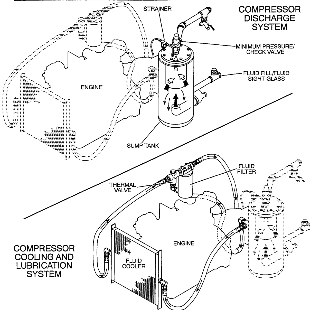
Figure 2-2 Compressor Discharge and Cooling and Lubrication System
