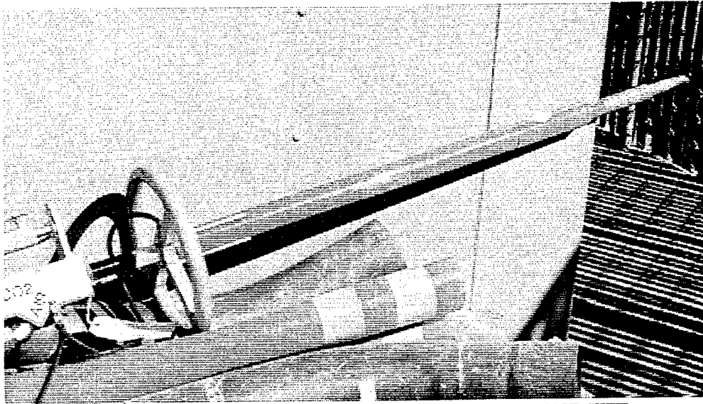
FIG. 8 ATTACH HOTSTICK & NOZZLE TIP
