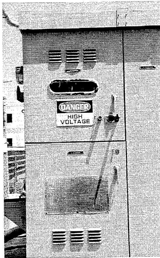
FIG. 9 TYPICAL LOAD INTERRUPTER SWITCHGEAR
