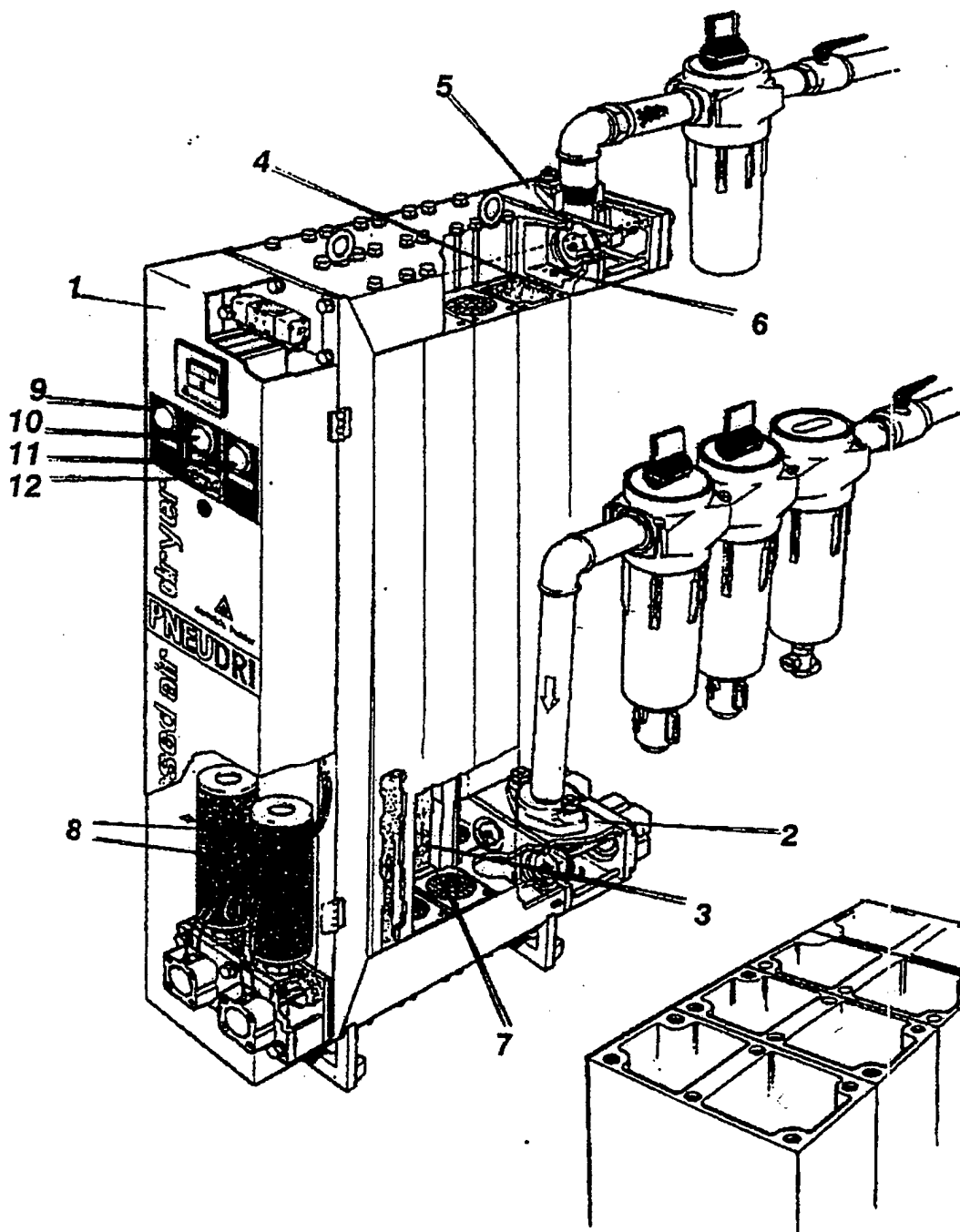
FIGURE 1 – TYPICAL HEATLESS DRYER CUTAWAY
