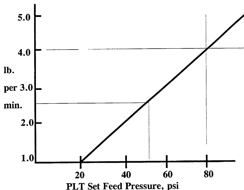
FIG. 16 - CO 2 PELLET DELIVERY RATE
