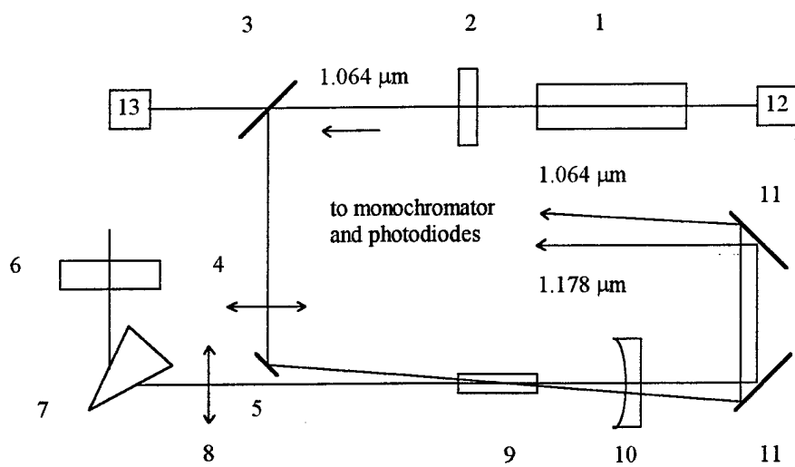
Fig. 5. Layout of \text{LiF:F}_2^- laser; uncollinear scheme of pumping.
