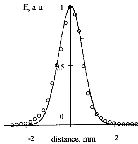
Fig. 4. Transverse distribution of the output beam energy.
