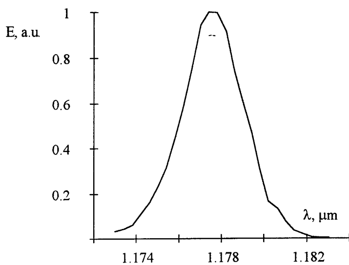
Fig. 8. Spectrum of LiF: F_2^- laser at pump pulse energy 4.5 mJ.
